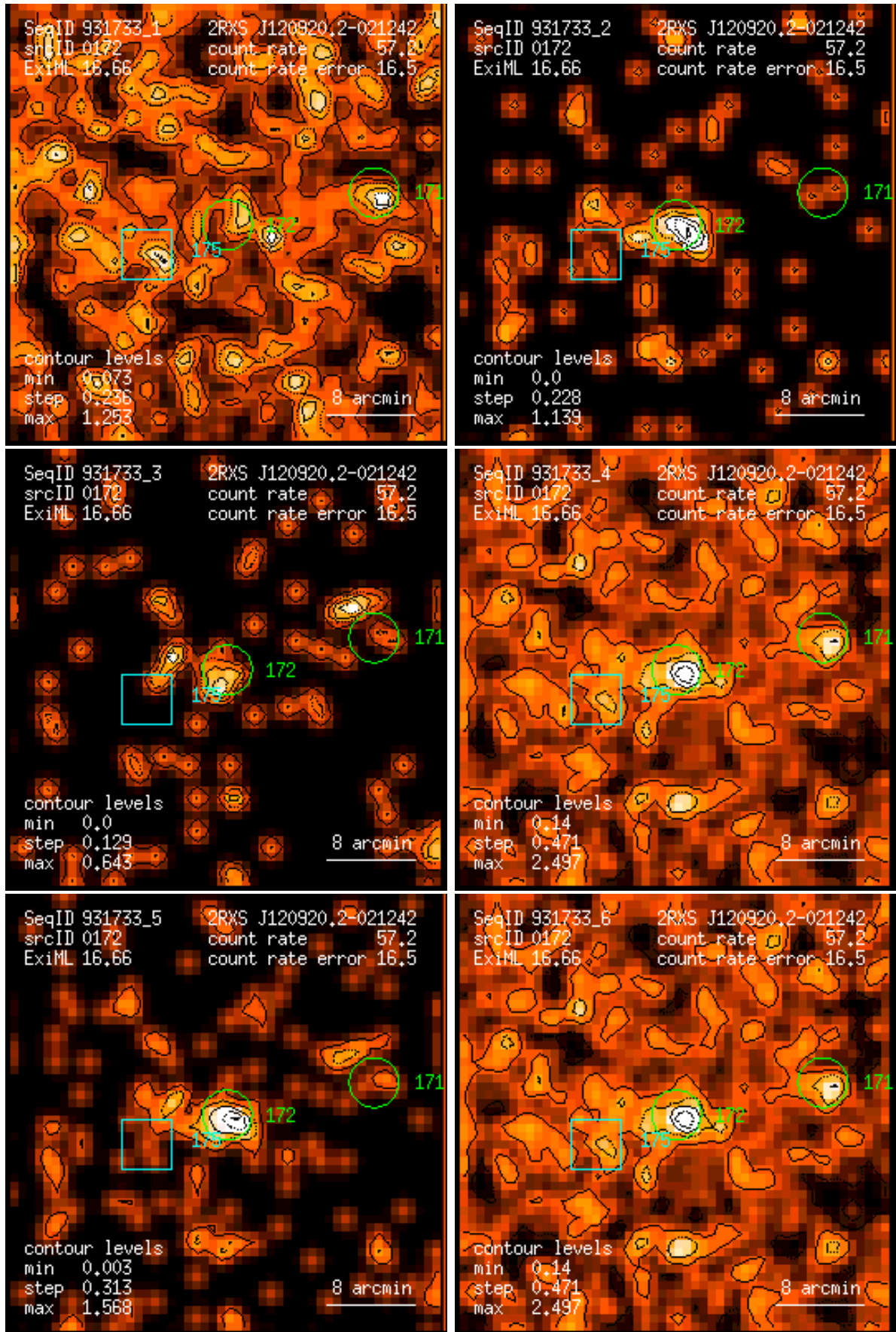
Figure 172: RASS 931733: detection 0172: band rate images, Gaussian filter: (1) PSPC channels 11 – 41, (2) 52 – 90, (3) 91 – 201, (4) 11 – 235, (5) 52 – 201, (6) 11 – 201. Broad band rates in counts/ks. Band rate contour levels in counts/ks/arcmin 2 .
