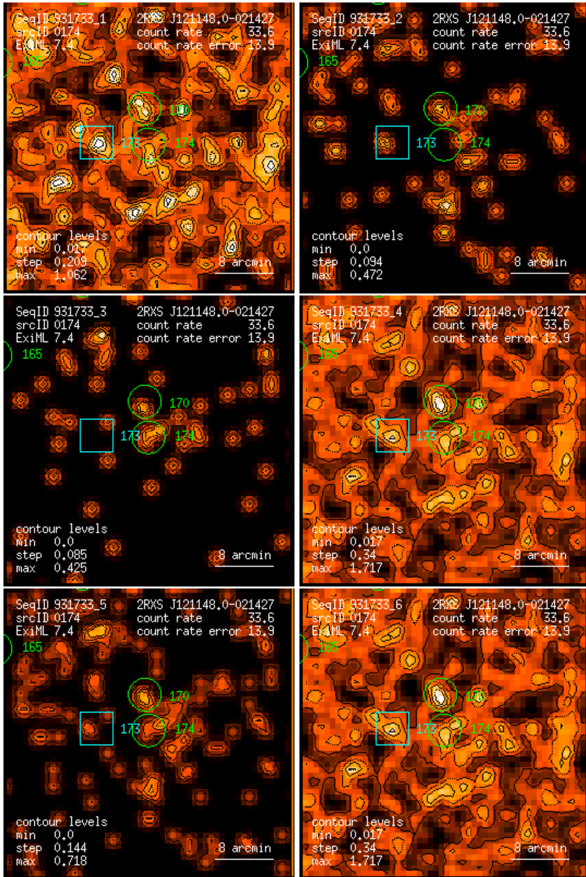
Figure 174: RASS 931733: detection 0174: band rate images, Gaussian filter: (1) PSPC channels 11 – 41, (2) 52 – 90, (3) 91 – 201, (4) 11 – 235, (5) 52 – 201, (6) 11 – 201. Broad band rates in counts/ks. Band rate contour levels in counts/ks/arcmin 2 .
