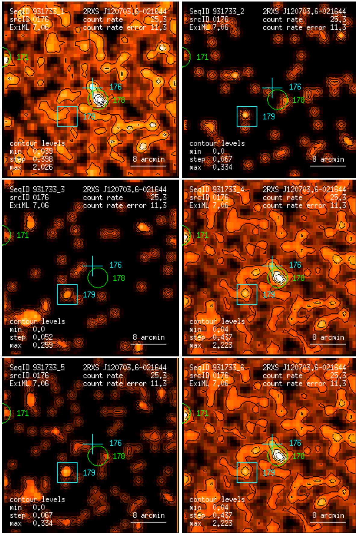
Figure 176: RASS 931733: detection 0176: band rate images, Gaussian filter: (1) PSPC channels 11 – 41, (2) 52 – 90, (3) 91 – 201, (4) 11 – 235, (5) 52 – 201, (6) 11 – 201. Broad band rates in counts/ks. Band rate contour levels in counts/ks/arcmin 2 .
