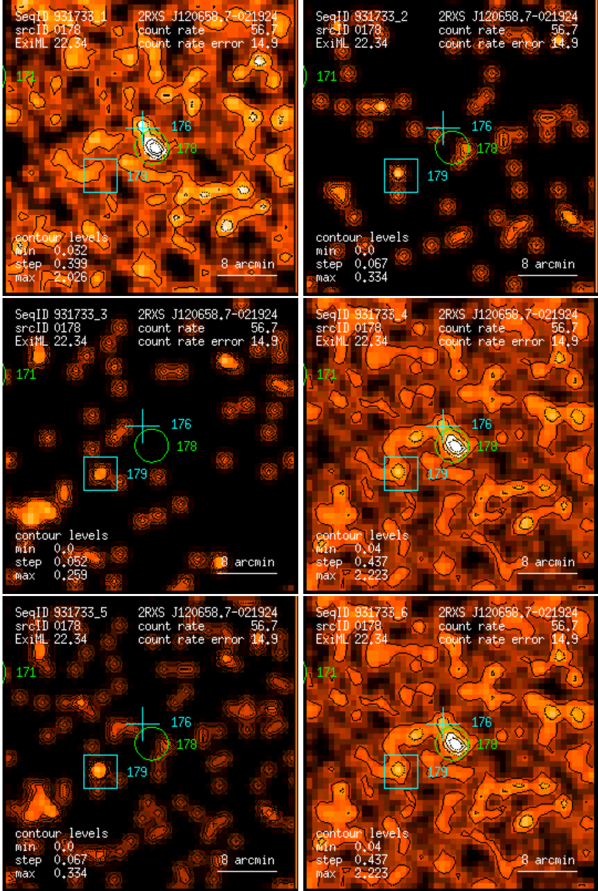
Figure 178: RASS 931733: detection 0178: band rate images, Gaussian filter: (1) PSPC channels 11 – 41, (2) 52 – 90, (3) 91 – 201, (4) 11 – 235, (5) 52 – 201, (6) 11 – 201. Broad band rates in counts/ks. Band rate contour levels in counts/ks/arcmin 2 .
