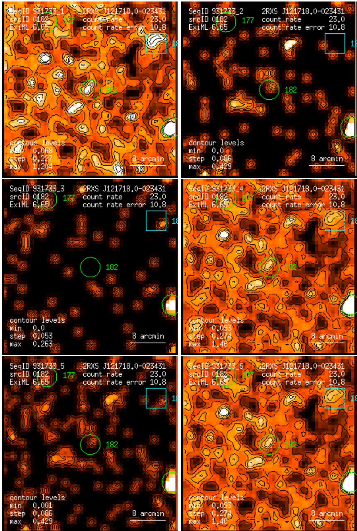
Figure 182: RASS 931733: detection 0182: band rate images, Gaussian filter: (1) PSPC channels 11 – 41, (2) 52 – 90, (3) 91 – 201, (4) 11 – 235, (5) 52 – 201, (6) 11 – 201. Broad band rates in counts/ks. Band rate contour levels in counts/ks/arcmin 2 .
