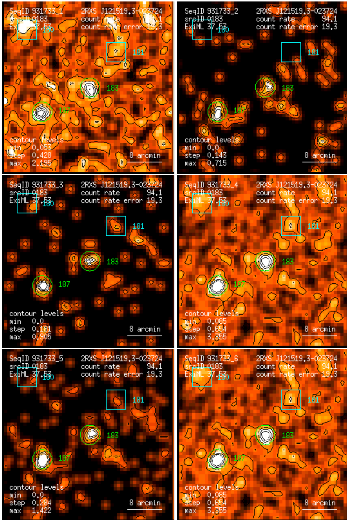
Figure 183: RASS 931733: detection 0183: band rate images, Gaussian filter: (1) PSPC channels 11 – 41, (2) 52 – 90, (3) 91 – 201, (4) 11 – 235, (5) 52 – 201, (6) 11 – 201. Broad band rates in counts/ks. Band rate contour levels in counts/ks/arcmin 2 .
