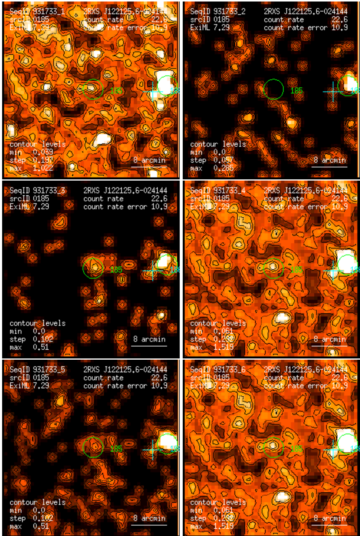
Figure 185: RASS 931733: detection 0185: band rate images, Gaussian filter: (1) PSPC channels 11 – 41, (2) 52 – 90, (3) 91 – 201, (4) 11 – 235, (5) 52 – 201, (6) 11 – 201. Broad band rates in counts/ks. Band rate contour levels in counts/ks/arcmin 2 .
