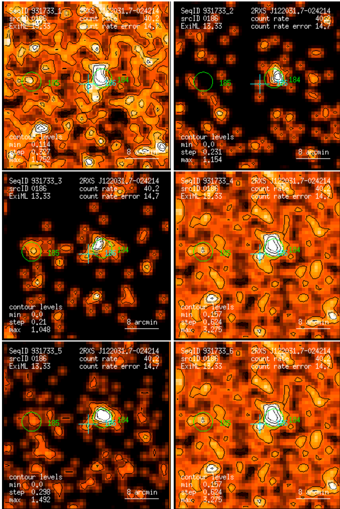
Figure 186: RASS 931733: detection 0186: band rate images, Gaussian filter: (1) PSPC channels 11 – 41, (2) 52 – 90, (3) 91 – 201, (4) 11 – 235, (5) 52 – 201, (6) 11 – 201. Broad band rates in counts/ks. Band rate contour levels in counts/ks/arcmin 2 .
