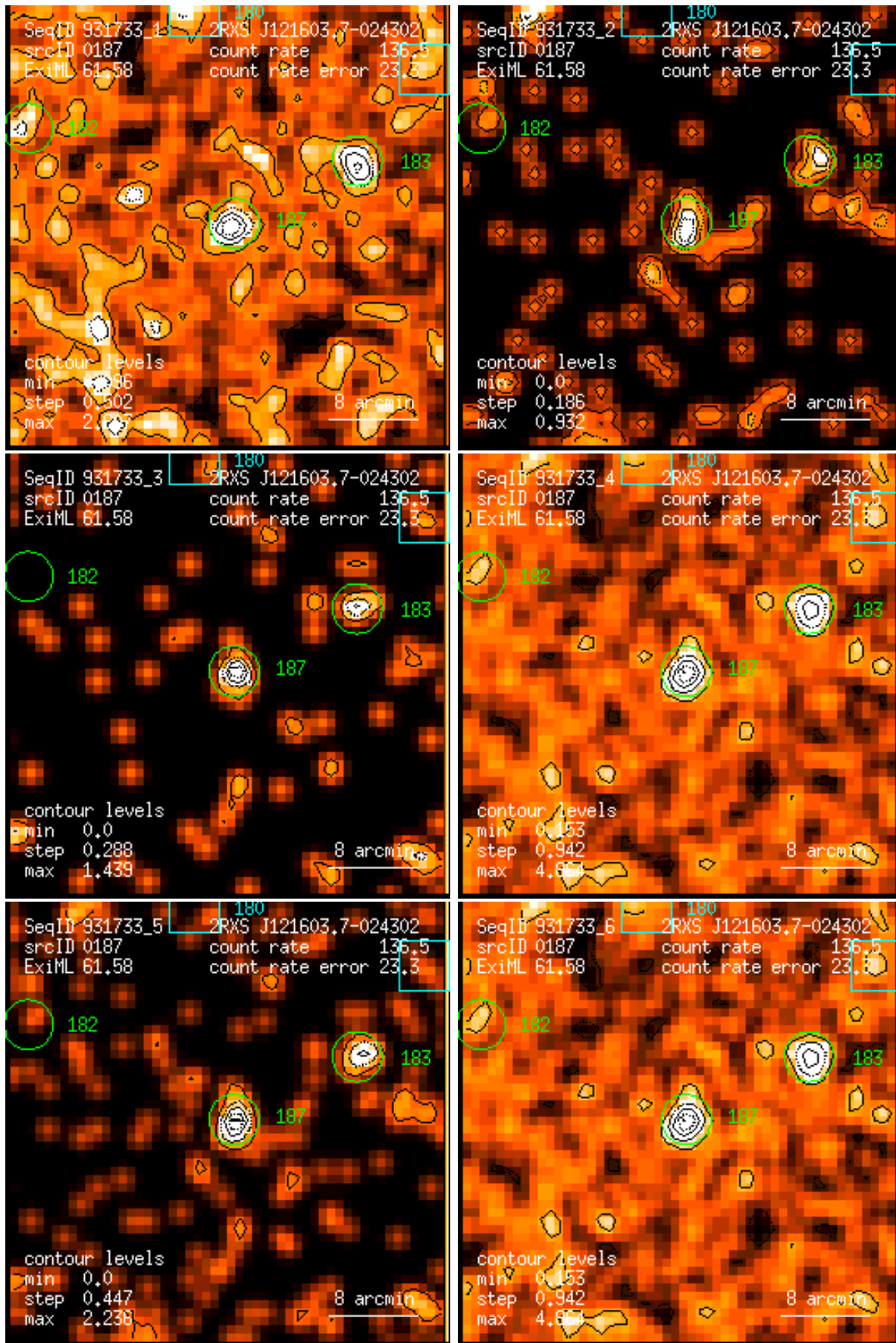
Figure 187: RASS 931733: detection 0187: band rate images, Gaussian filter: (1) PSPC channels 11 – 41, (2) 52 – 90, (3) 91 – 201, (4) 11 – 235, (5) 52 – 201, (6) 11 – 201. Broad band rates in counts/ks. Band rate contour levels in counts/ks/arcmin 2 .
