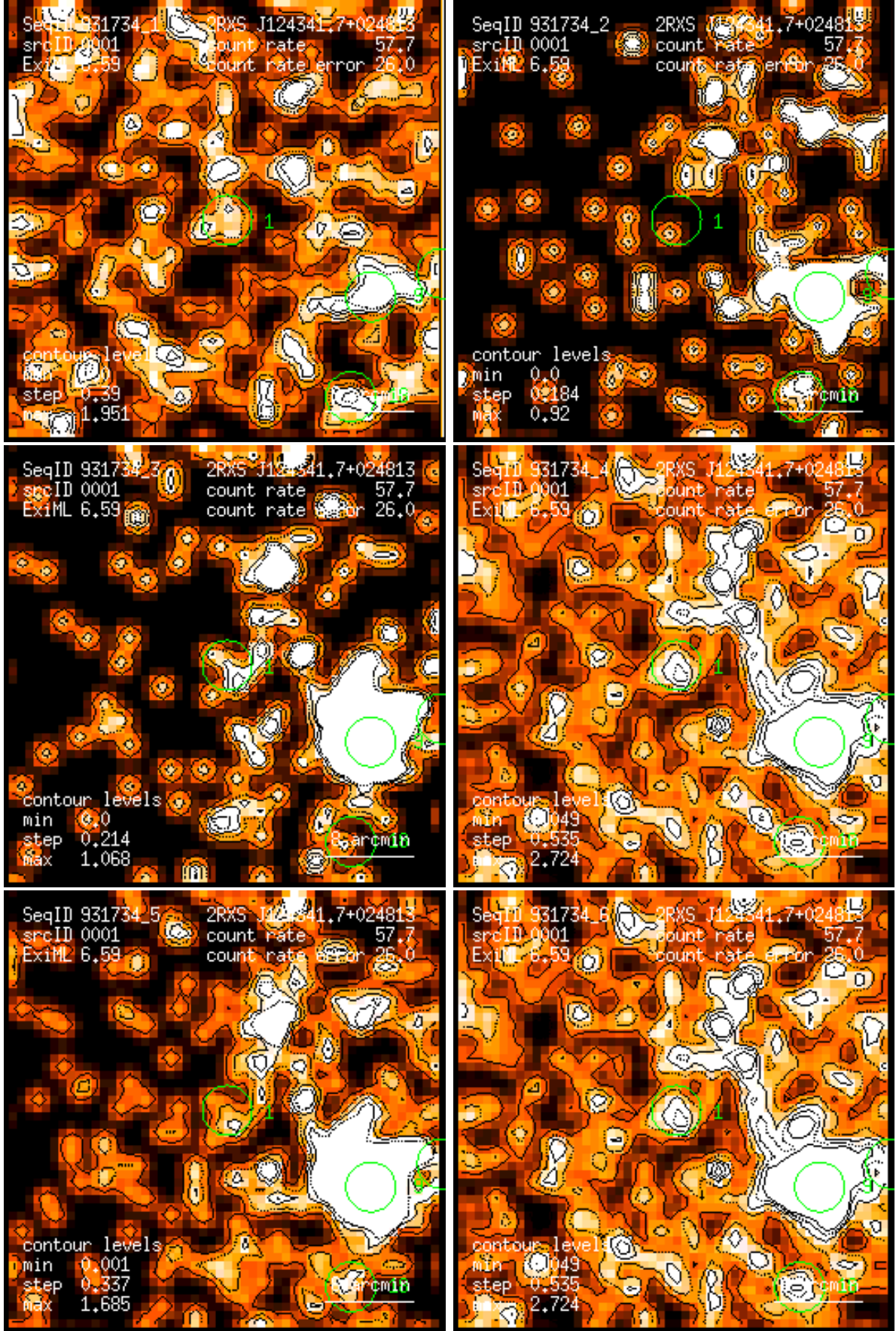
Figure 1: RASS 931734: detection 0001: band rate images, Gaussian filter: (1) PSPC channels 11 – 41, (2) 52 – 90, (3) 91 – 201, (4) 11 – 235, (5) 52 – 201, (6) 11 – 201. Broad band rates in counts/ks. Band rate contour levels in counts/ks/arcmin 2 .
