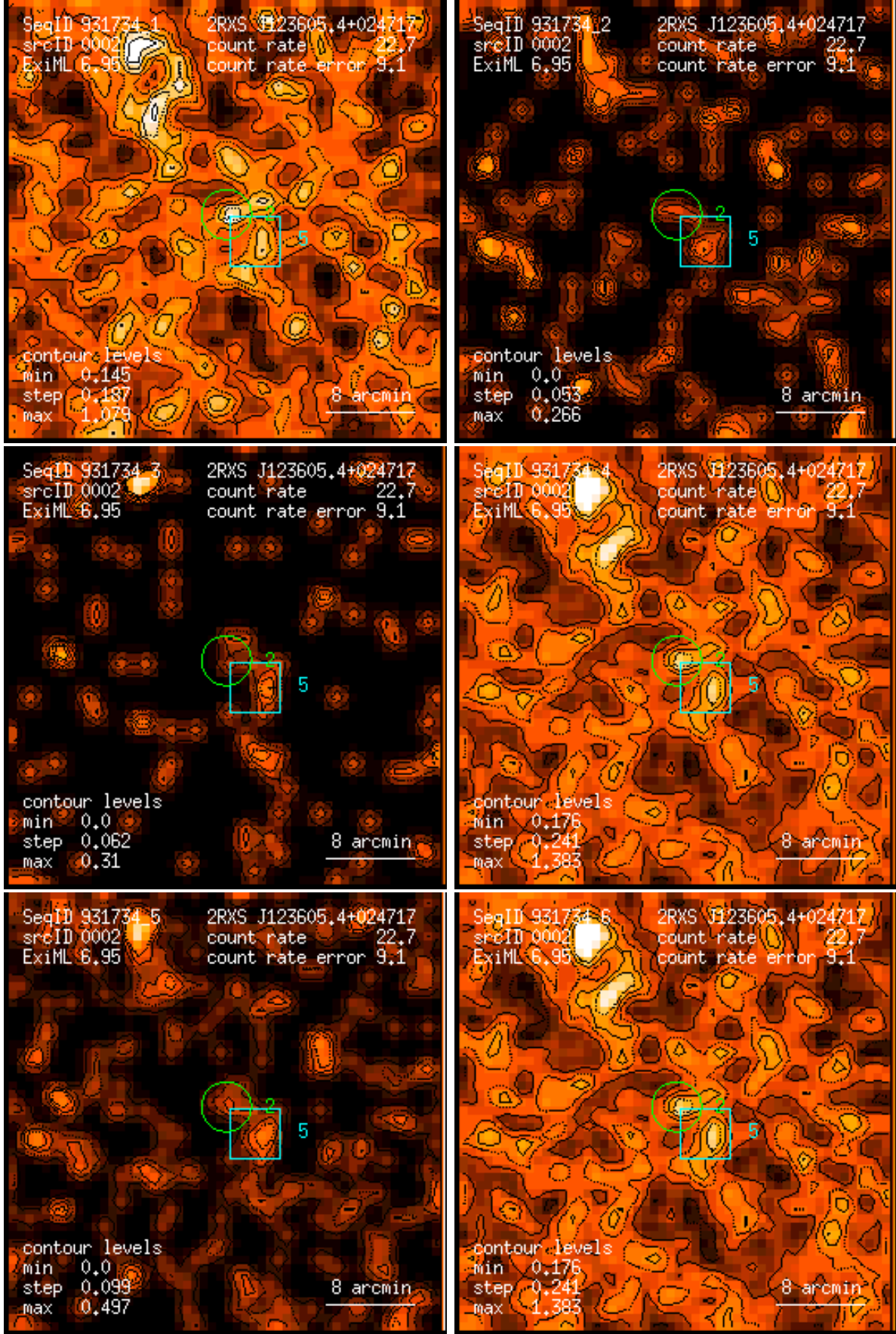
Figure 2: RASS 931734: detection 0002: band rate images, Gaussian filter: (1) PSPC channels 11 – 41, (2) 52 – 90, (3) 91 – 201, (4) 11 – 235, (5) 52 – 201, (6) 11 – 201. Broad band rates in counts/ks. Band rate contour levels in counts/ks/arcmin 2 .
