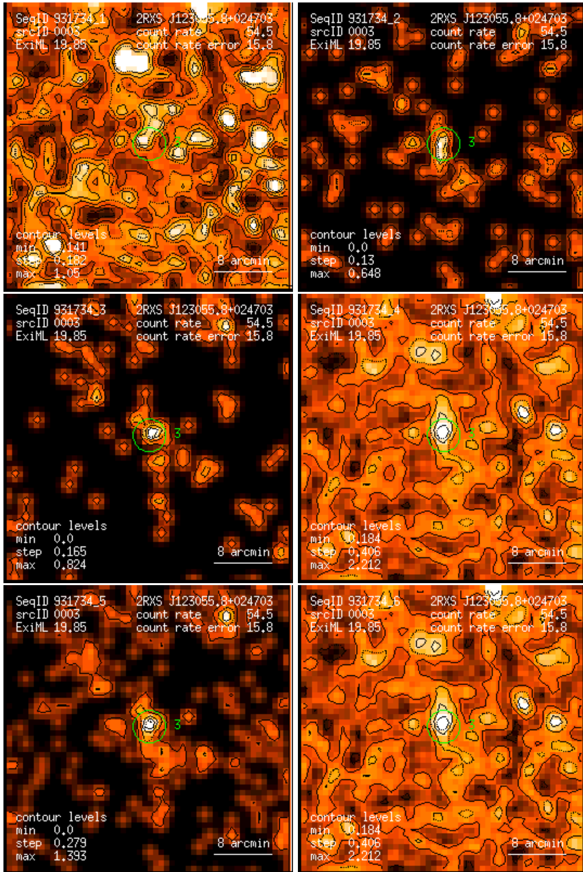
Figure 3: RASS 931734: detection 0003: band rate images, Gaussian filter: (1) PSPC channels 11 – 41, (2) 52 – 90, (3) 91 – 201, (4) 11 – 235, (5) 52 – 201, (6) 11 – 201. Broad band rates in counts/ks. Band rate contour levels in counts/ks/arcmin 2 .
