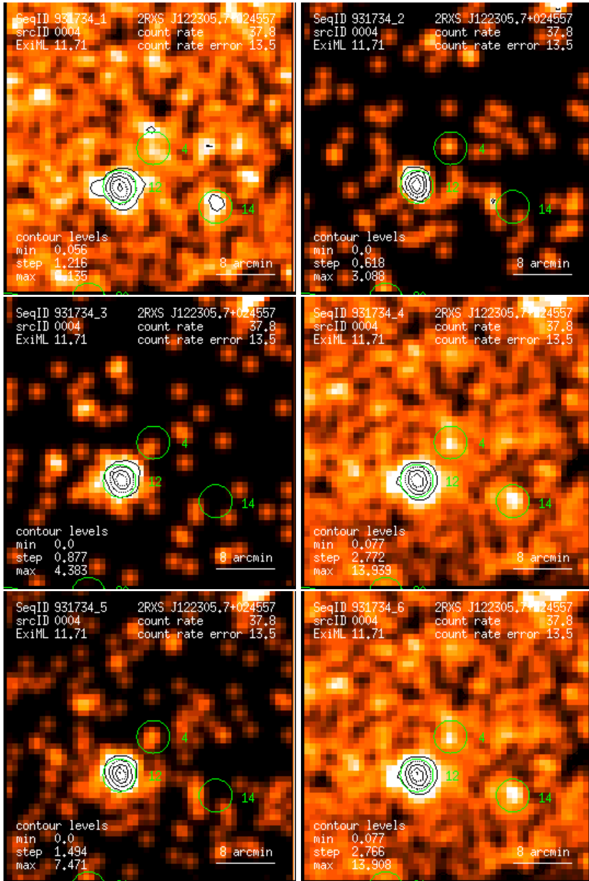
Figure 4: RASS 931734: detection 0004: band rate images, Gaussian filter: (1) PSPC channels 11 – 41, (2) 52 – 90, (3) 91 – 201, (4) 11 – 235, (5) 52 – 201, (6) 11 – 201. Broad band rates in counts/ks. Band rate contour levels in counts/ks/arcmin 2 .
