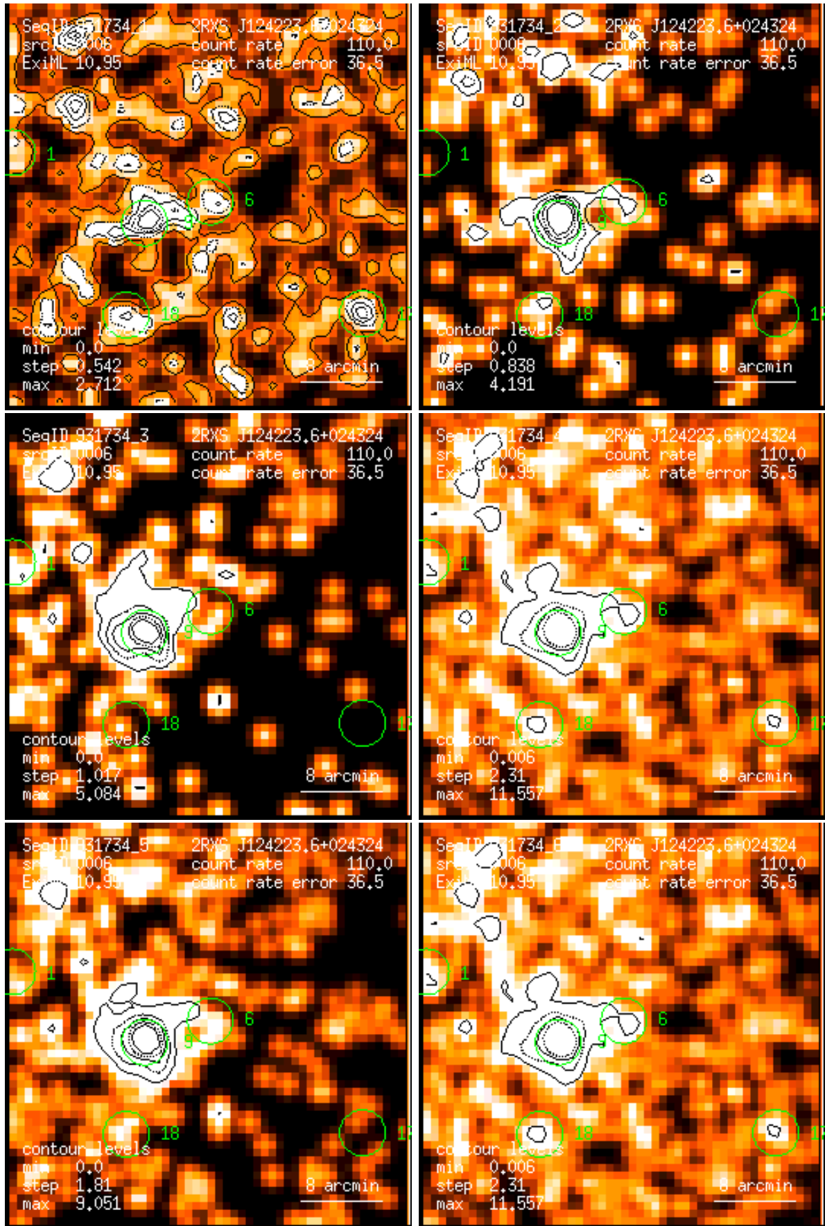
Figure 6: RASS 931734: detection 0006: band rate images, Gaussian filter: (1) PSPC channels 11 – 41, (2) 52 – 90, (3) 91 – 201, (4) 11 – 235, (5) 52 – 201, (6) 11 – 201. Broad band rates in counts/ks. Band rate contour levels in counts/ks/arcmin 2 .
