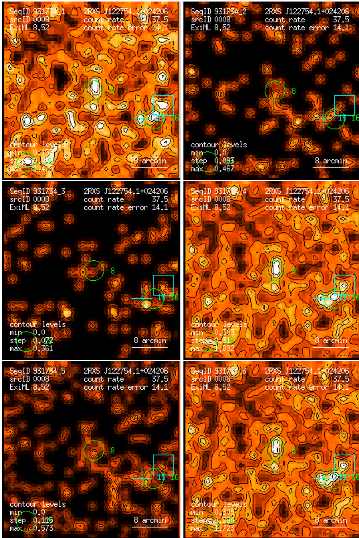
Figure 8: RASS 931734: detection 0008: band rate images, Gaussian filter: (1) PSPC channels 11 – 41, (2) 52 – 90, (3) 91 – 201, (4) 11 – 235, (5) 52 – 201, (6) 11 – 201. Broad band rates in counts/ks. Band rate contour levels in counts/ks/arcmin 2 .
