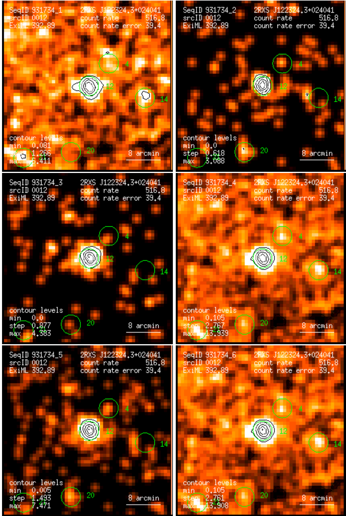
Figure 12: RASS 931734: detection 0012: band rate images, Gaussian filter: (1) PSPC channels 11 – 41, (2) 52 – 90, (3) 91 – 201, (4) 11 – 235, (5) 52 – 201, (6) 11 – 201. Broad band rates in counts/ks. Band rate contour levels in counts/ks/arcmin 2 .
