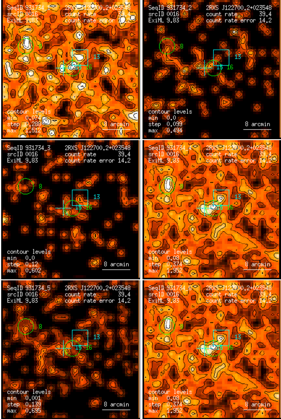
Figure 16: RASS 931734: detection 0016: band rate images, Gaussian filter: (1) PSPC channels 11 – 41, (2) 52 – 90, (3) 91 – 201, (4) 11 – 235, (5) 52 – 201, (6) 11 – 201. Broad band rates in counts/ks. Band rate contour levels in counts/ks/arcmin 2 .
