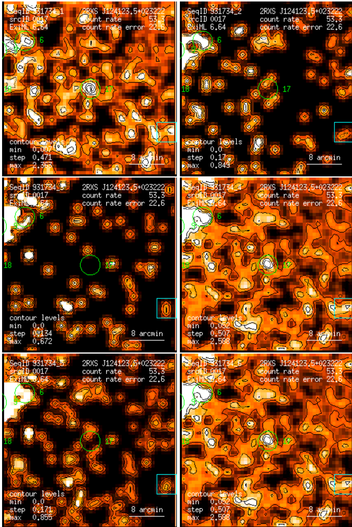
Figure 17: RASS 931734: detection 0017: band rate images, Gaussian filter: (1) PSPC channels 11 – 41, (2) 52 – 90, (3) 91 – 201, (4) 11 – 235, (5) 52 – 201, (6) 11 – 201. Broad band rates in counts/ks. Band rate contour levels in counts/ks/arcmin 2 .
