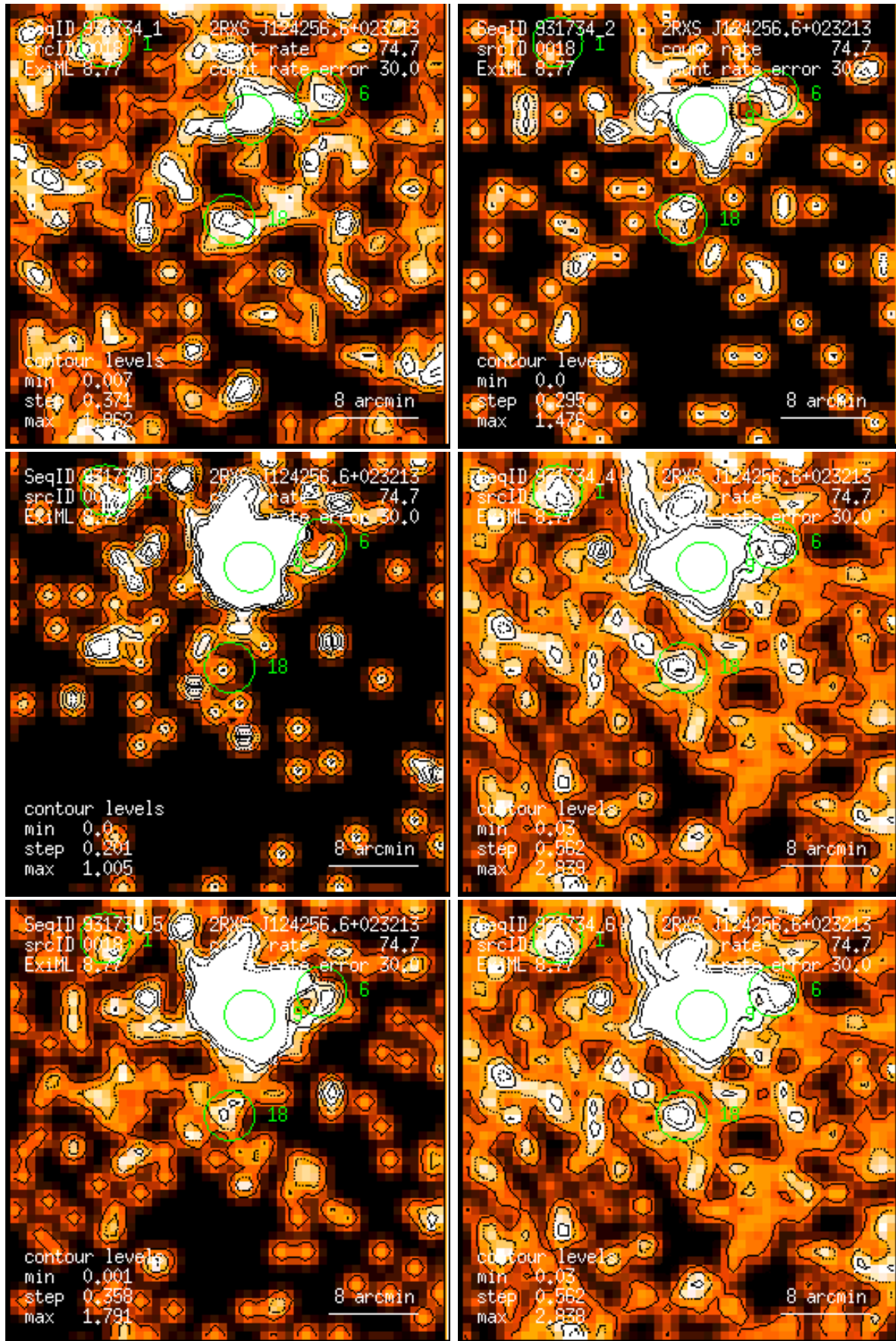
Figure 18: RASS 931734: detection 0018: band rate images, Gaussian filter: (1) PSPC channels 11 – 41, (2) 52 – 90, (3) 91 – 201, (4) 11 – 235, (5) 52 – 201, (6) 11 – 201. Broad band rates in counts/ks. Band rate contour levels in counts/ks/arcmin 2 .
