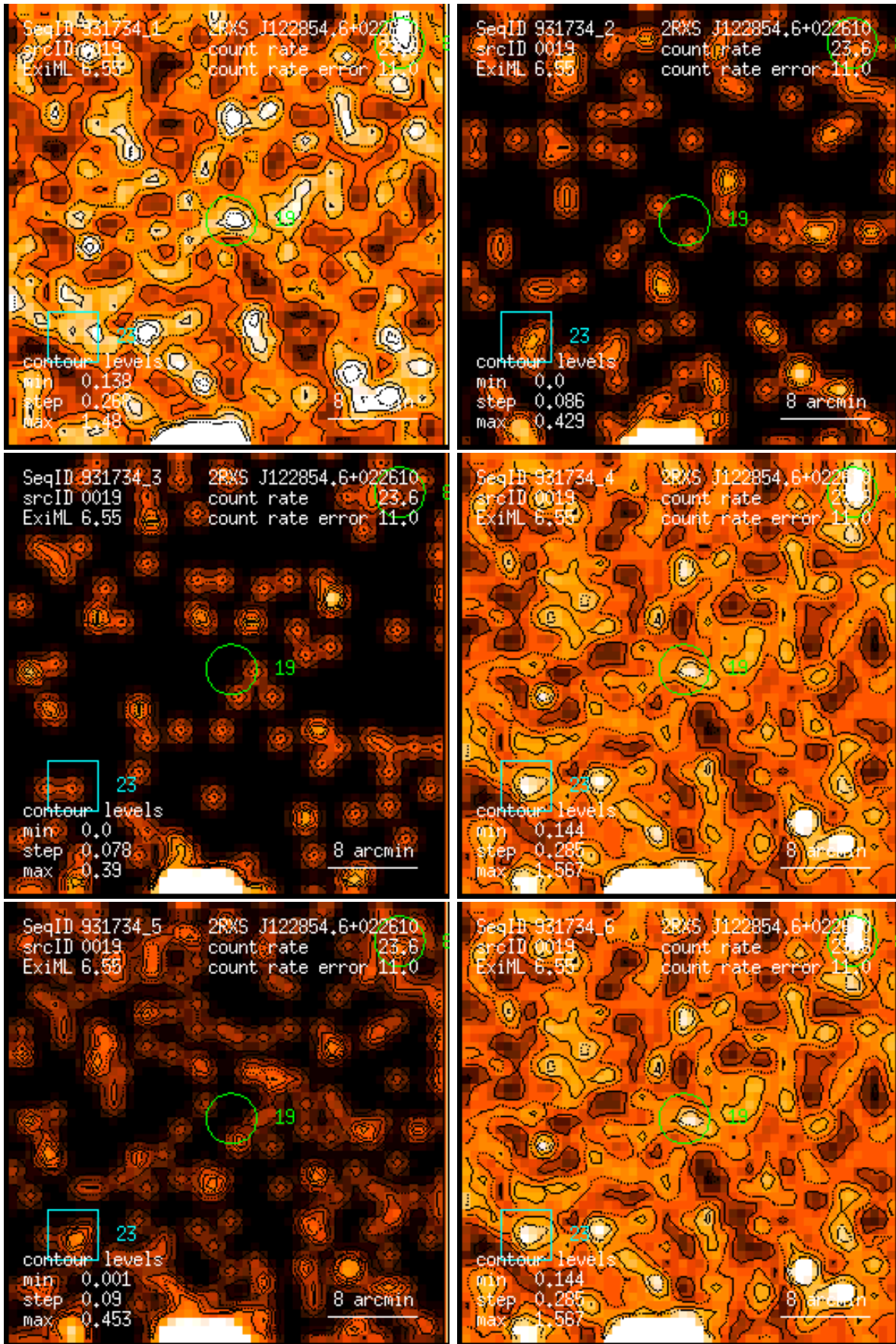
Figure 19: RASS 931734: detection 0019: band rate images, Gaussian filter: (1) PSPC channels 11 – 41, (2) 52 – 90, (3) 91 – 201, (4) 11 – 235, (5) 52 – 201, (6) 11 – 201. Broad band rates in counts/ks. Band rate contour levels in counts/ks/arcmin 2 .
