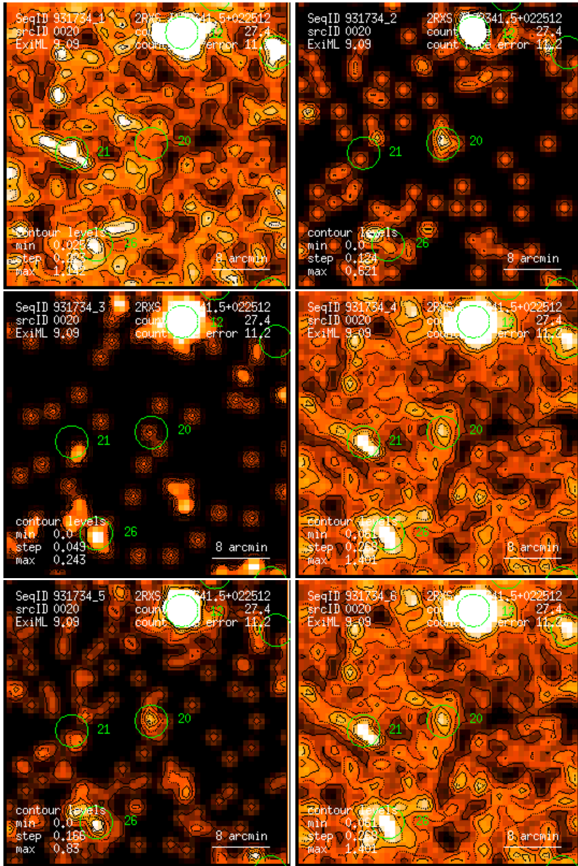
Figure 20: RASS 931734: detection 0020: band rate images, Gaussian filter: (1) PSPC channels 11 – 41, (2) 52 – 90, (3) 91 – 201, (4) 11 – 235, (5) 52 – 201, (6) 11 – 201. Broad band rates in counts/ks. Band rate contour levels in counts/ks/arcmin 2 .
