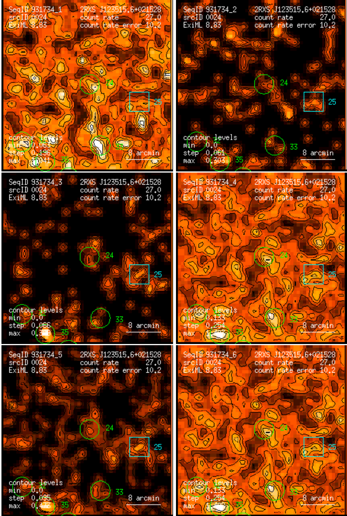
Figure 24: RASS 931734: detection 0024: band rate images, Gaussian filter: (1) PSPC channels 11 – 41, (2) 52 – 90, (3) 91 – 201, (4) 11 – 235, (5) 52 – 201, (6) 11 – 201. Broad band rates in counts/ks. Band rate contour levels in counts/ks/arcmin 2 .
