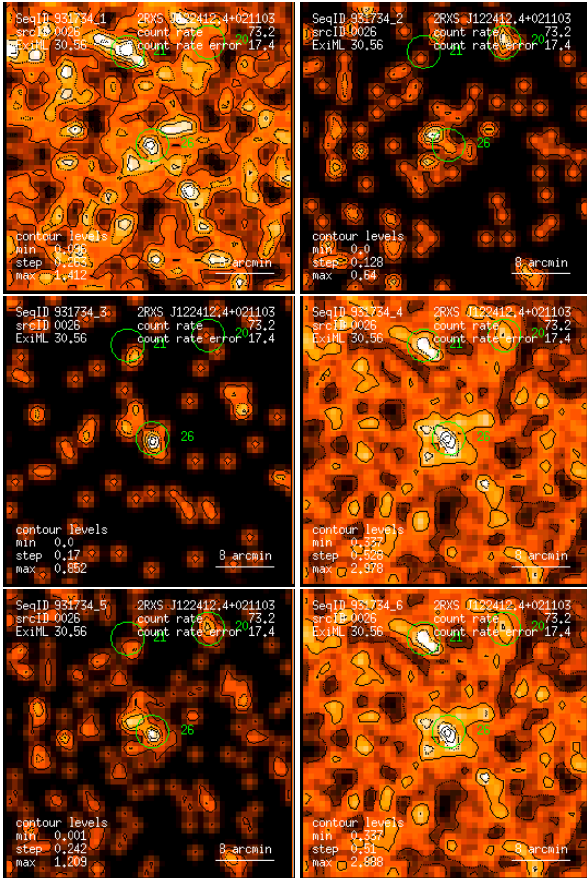
Figure 26: RASS 931734: detection 0026: band rate images, Gaussian filter: (1) PSPC channels 11 – 41, (2) 52 – 90, (3) 91 – 201, (4) 11 – 235, (5) 52 – 201, (6) 11 – 201. Broad band rates in counts/ks. Band rate contour levels in counts/ks/arcmin 2 .
