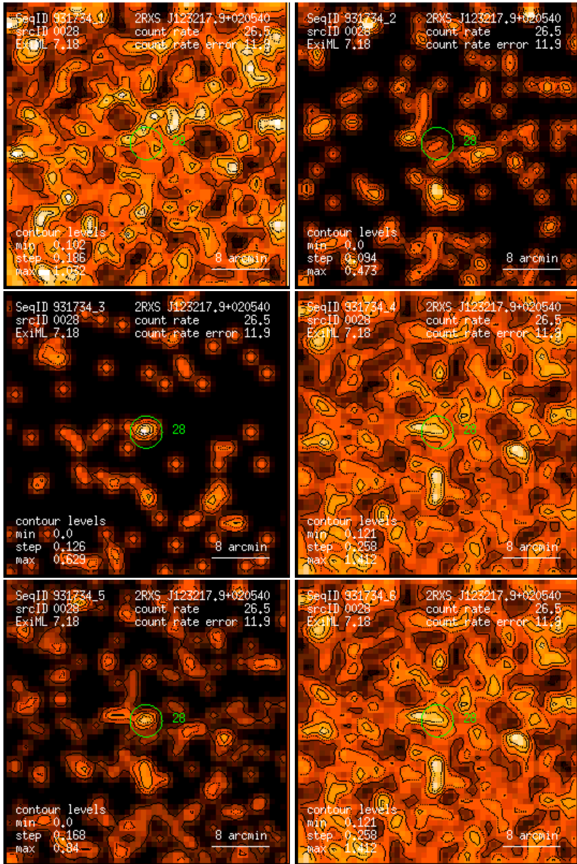
Figure 28: RASS 931734: detection 0028: band rate images, Gaussian filter: (1) PSPC channels 11 – 41, (2) 52 – 90, (3) 91 – 201, (4) 11 – 235, (5) 52 – 201, (6) 11 – 201. Broad band rates in counts/ks. Band rate contour levels in counts/ks/arcmin 2 .
