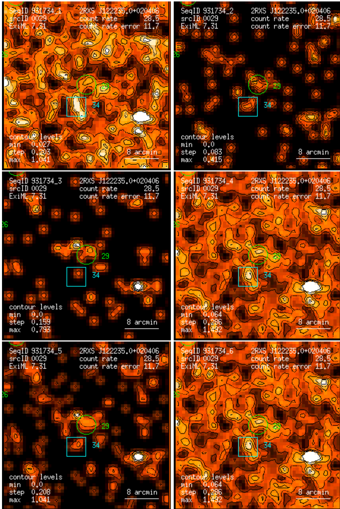
Figure 29: RASS 931734: detection 0029: band rate images, Gaussian filter: (1) PSPC channels 11 – 41, (2) 52 – 90, (3) 91 – 201, (4) 11 – 235, (5) 52 – 201, (6) 11 – 201. Broad band rates in counts/ks. Band rate contour levels in counts/ks/arcmin 2 .
