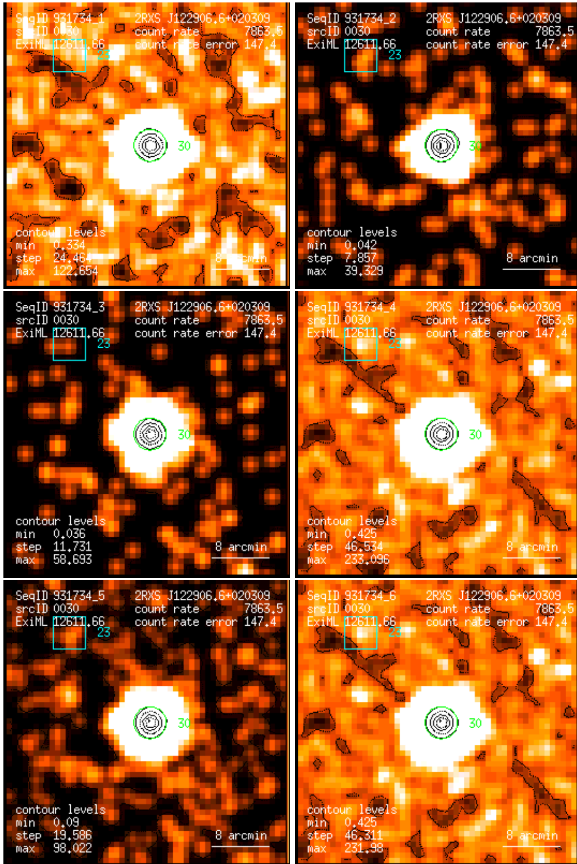
Figure 30: RASS 931734: detection 0030: band rate images, Gaussian filter: (1) PSPC channels 11 – 41, (2) 52 – 90, (3) 91 – 201, (4) 11 – 235, (5) 52 – 201, (6) 11 – 201. Broad band rates in counts/ks. Band rate contour levels in counts/ks/arcmin 2 .
