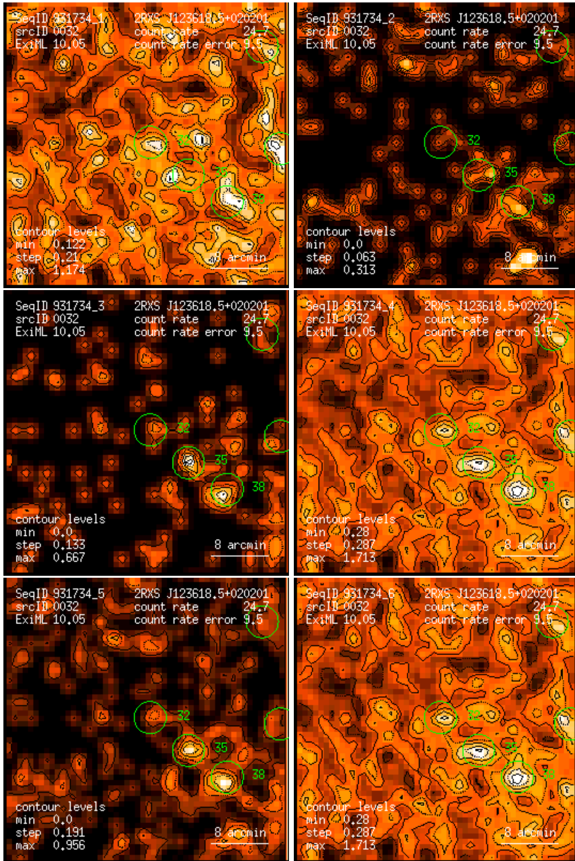
Figure 32: RASS 931734: detection 0032: band rate images, Gaussian filter: (1) PSPC channels 11 – 41, (2) 52 – 90, (3) 91 – 201, (4) 11 – 235, (5) 52 – 201, (6) 11 – 201. Broad band rates in counts/ks. Band rate contour levels in counts/ks/arcmin 2 .
