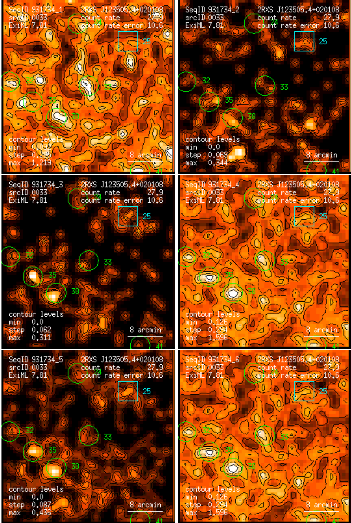
Figure 33: RASS 931734: detection 0033: band rate images, Gaussian filter: (1) PSPC channels 11 – 41, (2) 52 – 90, (3) 91 – 201, (4) 11 – 235, (5) 52 – 201, (6) 11 – 201. Broad band rates in counts/ks. Band rate contour levels in counts/ks/arcmin 2 .
