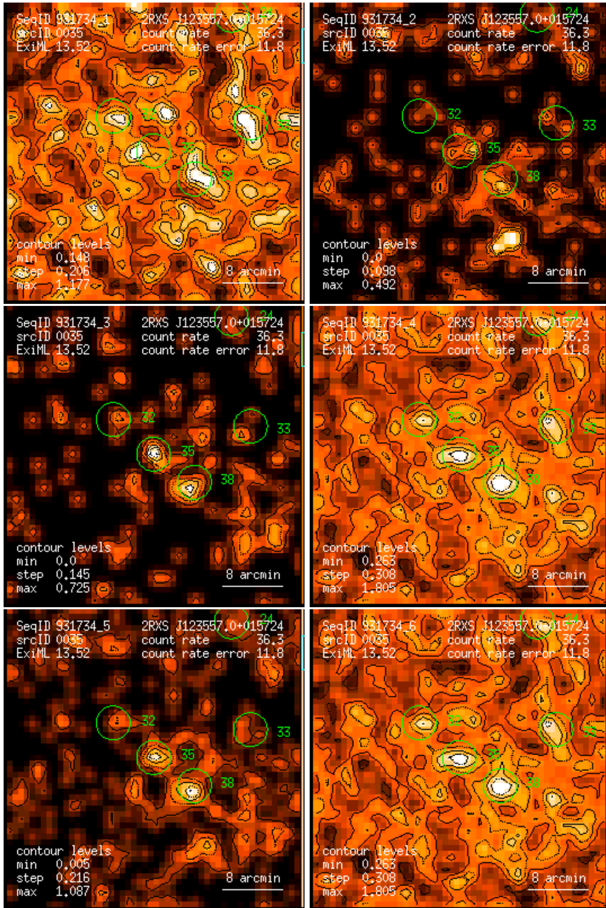
Figure 35: RASS 931734: detection 0035: band rate images, Gaussian filter: (1) PSPC channels 11 – 41, (2) 52 – 90, (3) 91 – 201, (4) 11 – 235, (5) 52 – 201, (6) 11 – 201. Broad band rates in counts/ks. Band rate contour levels in counts/ks/arcmin 2 .
