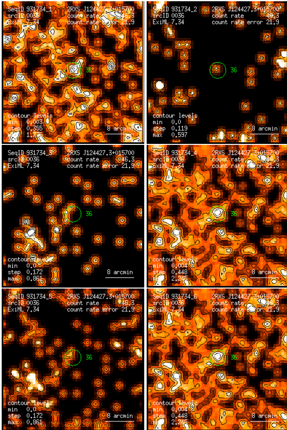
Figure 36: RASS 931734: detection 0036: band rate images, Gaussian filter: (1) PSPC channels 11 – 41, (2) 52 – 90, (3) 91 – 201, (4) 11 – 235, (5) 52 – 201, (6) 11 – 201. Broad band rates in counts/ks. Band rate contour levels in counts/ks/arcmin 2 .
