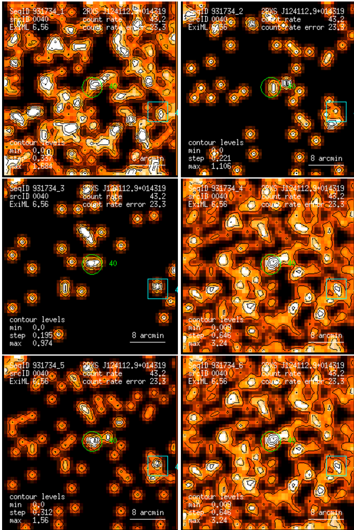
Figure 40: RASS 931734: detection 0040: band rate images, Gaussian filter: (1) PSPC channels 11 – 41, (2) 52 – 90, (3) 91 – 201, (4) 11 – 235, (5) 52 – 201, (6) 11 – 201. Broad band rates in counts/ks. Band rate contour levels in counts/ks/arcmin 2 .
