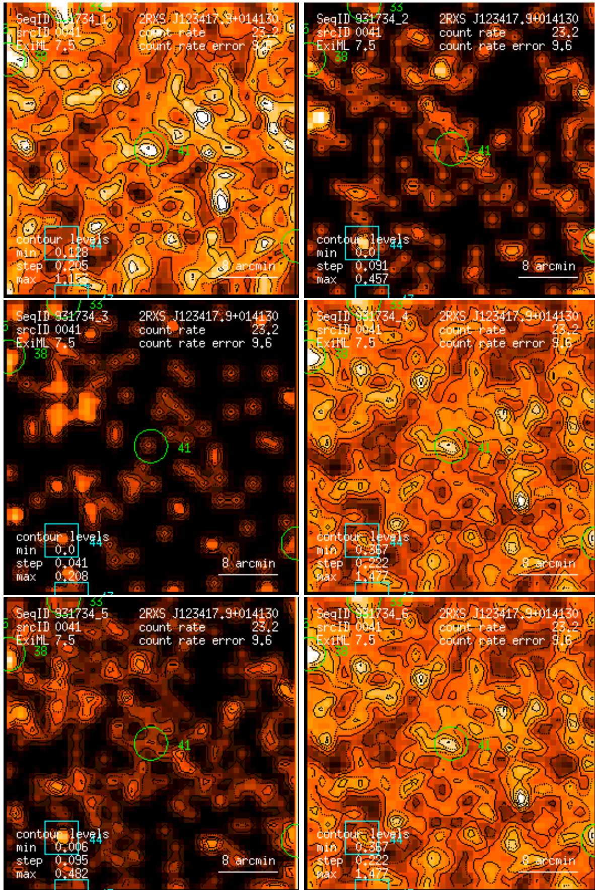
Figure 41: RASS 931734: detection 0041: band rate images, Gaussian filter: (1) PSPC channels 11 – 41, (2) 52 – 90, (3) 91 – 201, (4) 11 – 235, (5) 52 – 201, (6) 11 – 201. Broad band rates in counts/ks. Band rate contour levels in counts/ks/arcmin 2 .
