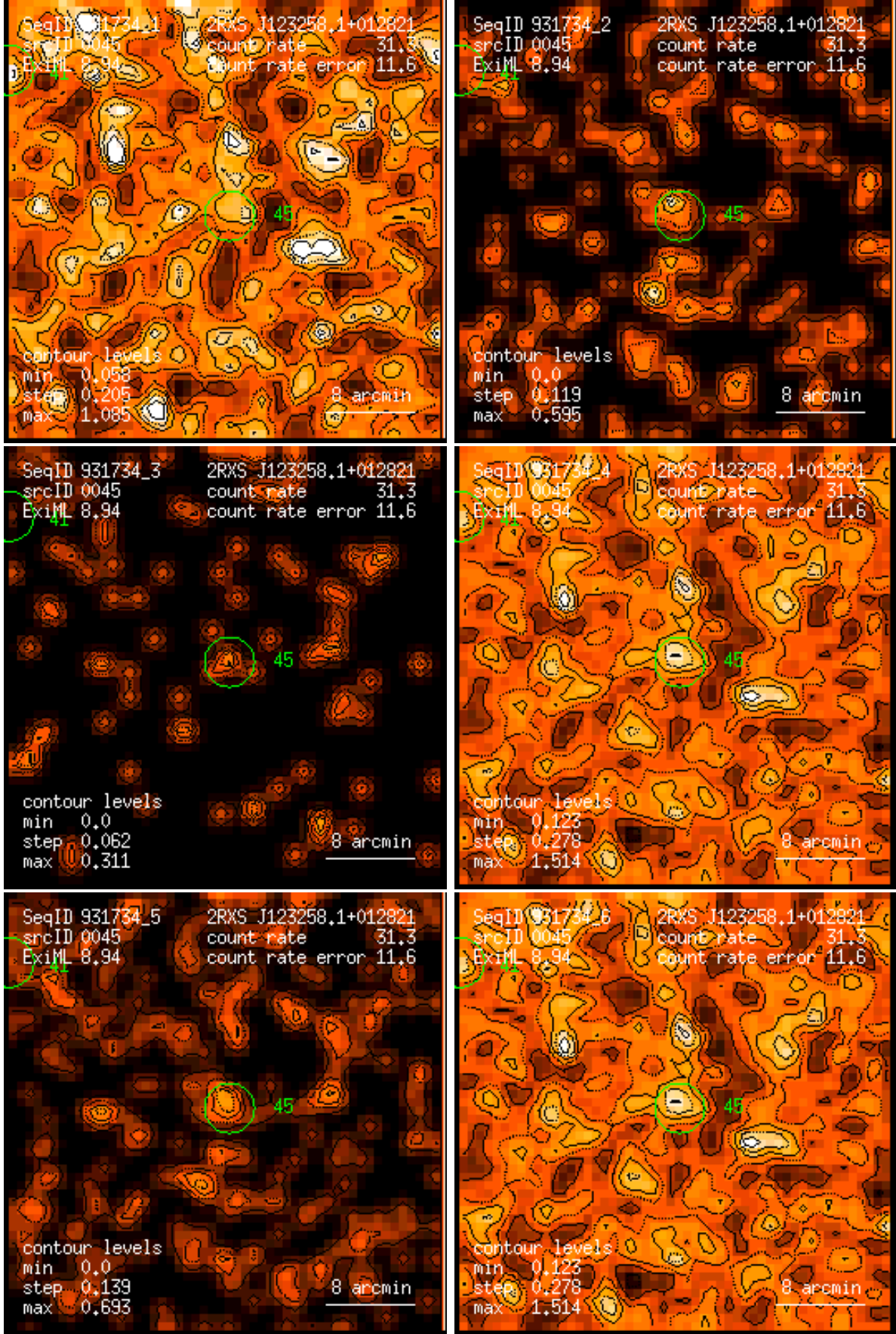
Figure 45: RASS 931734: detection 0045: band rate images, Gaussian filter: (1) PSPC channels 11 – 41, (2) 52 – 90, (3) 91 – 201, (4) 11 – 235, (5) 52 – 201, (6) 11 – 201. Broad band rates in counts/ks. Band rate contour levels in counts/ks/arcmin 2 .
