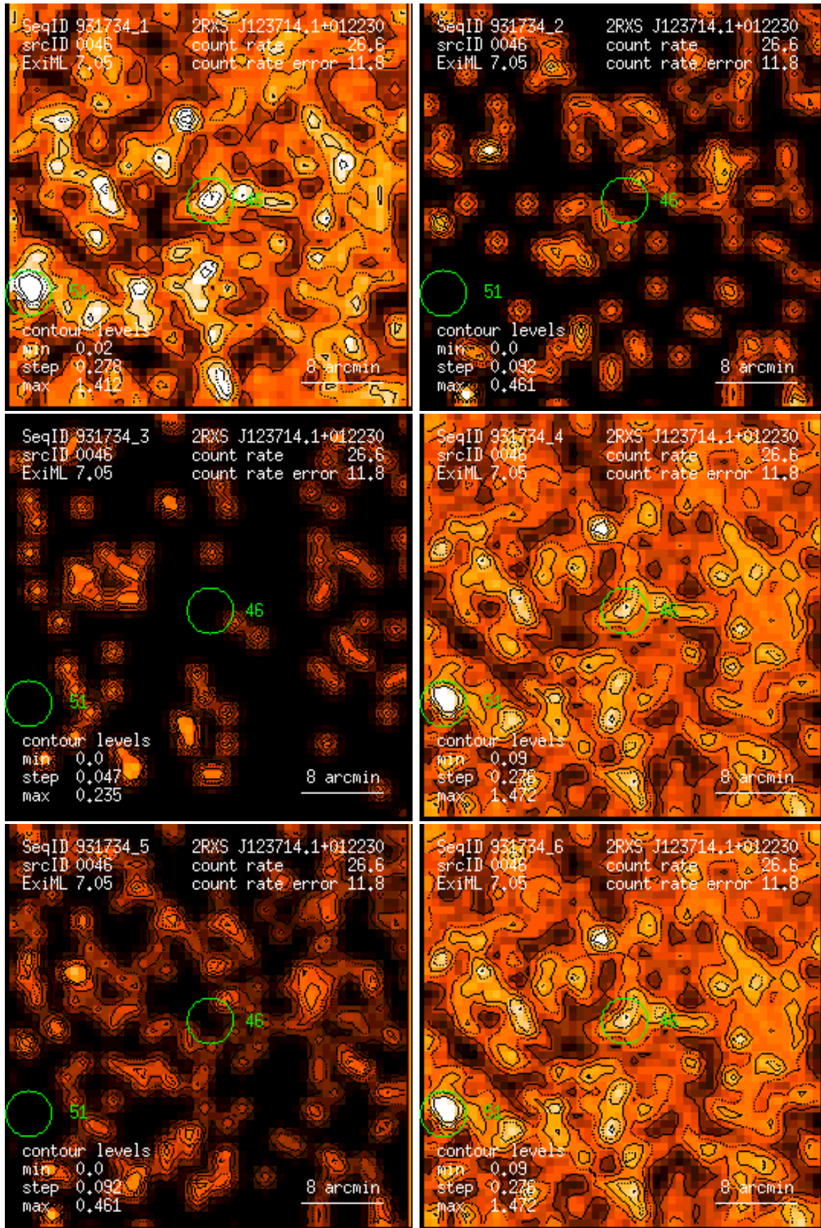
Figure 46: RASS 931734: detection 0046: band rate images, Gaussian filter: (1) PSPC channels 11 – 41, (2) 52 – 90, (3) 91 – 201, (4) 11 – 235, (5) 52 – 201, (6) 11 – 201. Broad band rates in counts/ks. Band rate contour levels in counts/ks/arcmin 2 .
