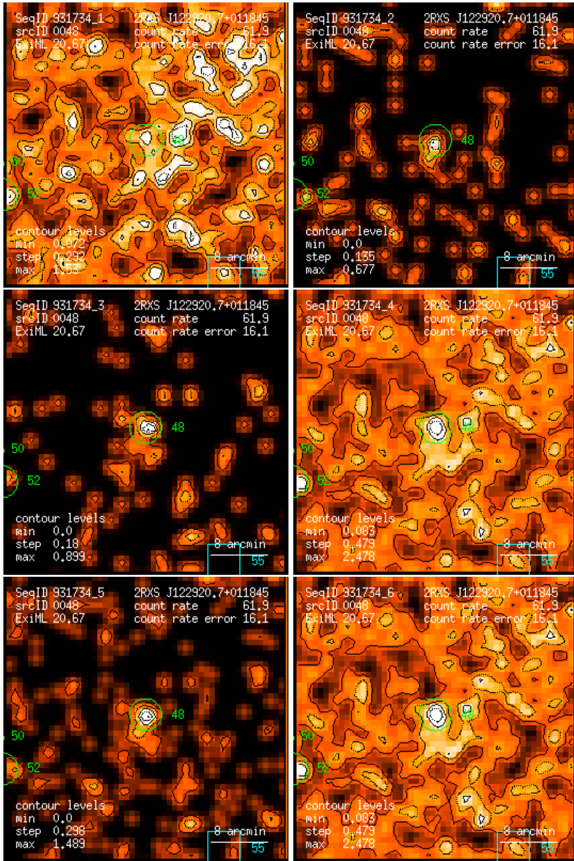
Figure 48: RASS 931734: detection 0048: band rate images, Gaussian filter: (1) PSPC channels 11 – 41, (2) 52 – 90, (3) 91 – 201, (4) 11 – 235, (5) 52 – 201, (6) 11 – 201. Broad band rates in counts/ks. Band rate contour levels in counts/ks/arcmin 2 .
