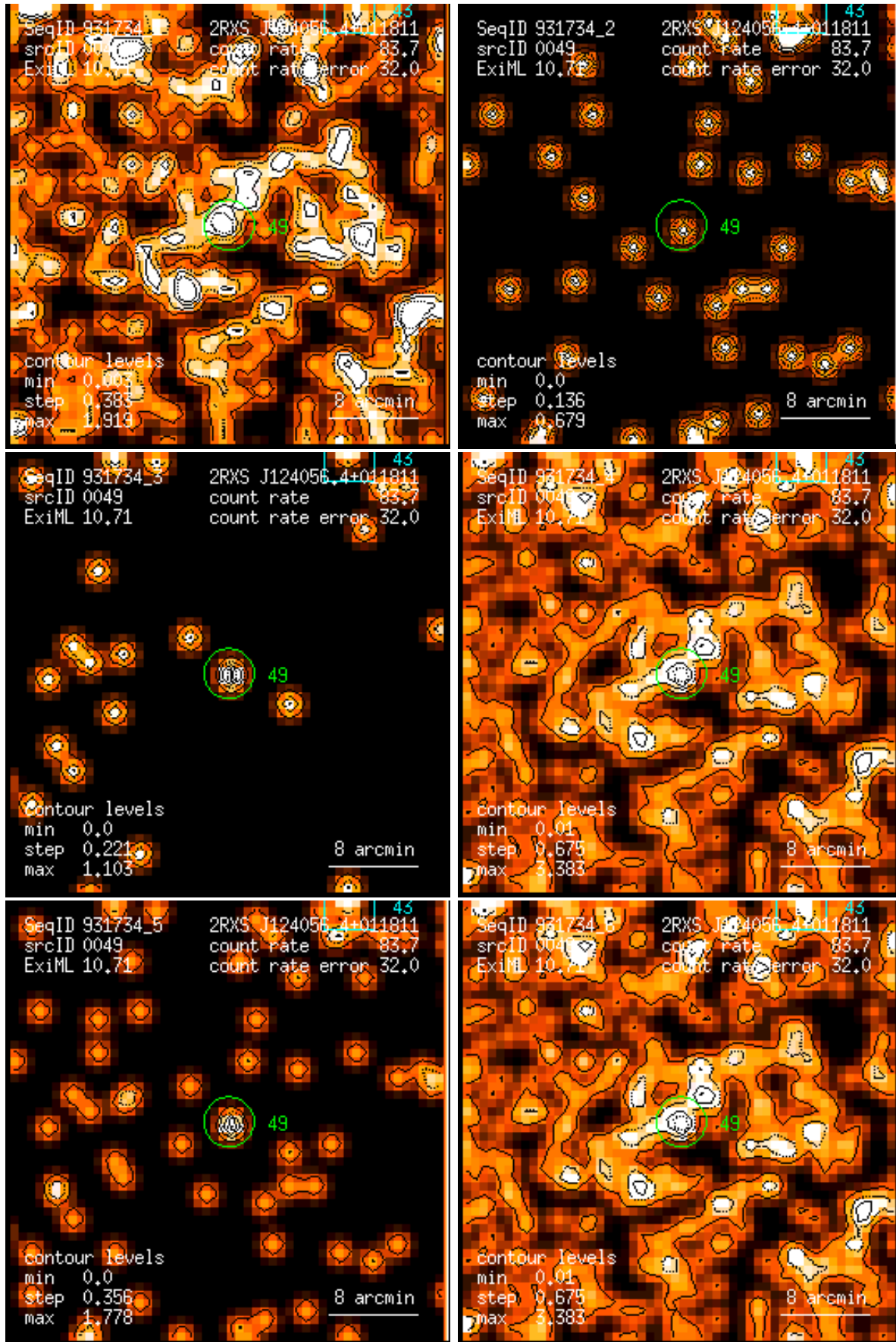
Figure 49: RASS 931734: detection 0049: band rate images, Gaussian filter: (1) PSPC channels 11 – 41, (2) 52 – 90, (3) 91 – 201, (4) 11 – 235, (5) 52 – 201, (6) 11 – 201. Broad band rates in counts/ks. Band rate contour levels in counts/ks/arcmin 2 .
