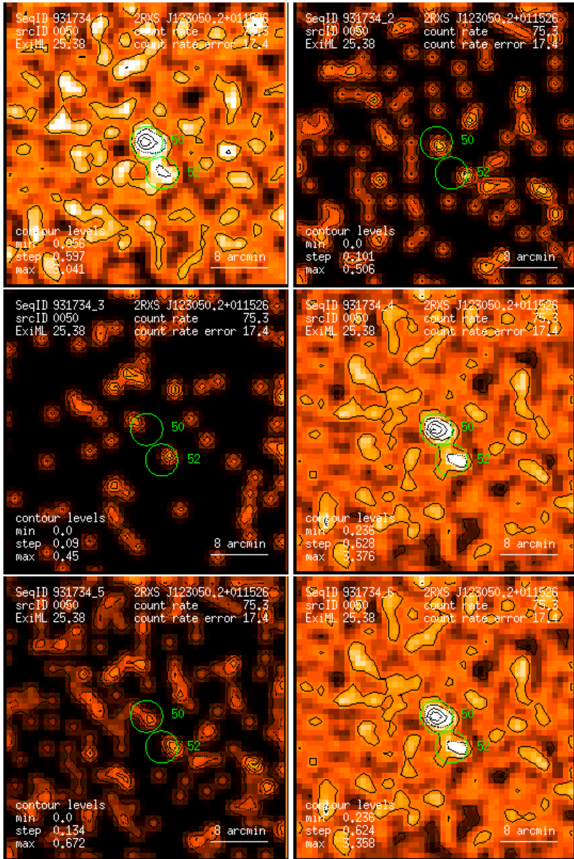
Figure 50: RASS 931734: detection 0050: band rate images, Gaussian filter: (1) PSPC channels 11 – 41, (2) 52 – 90, (3) 91 – 201, (4) 11 – 235, (5) 52 – 201, (6) 11 – 201. Broad band rates in counts/ks. Band rate contour levels in counts/ks/arcmin 2 .
