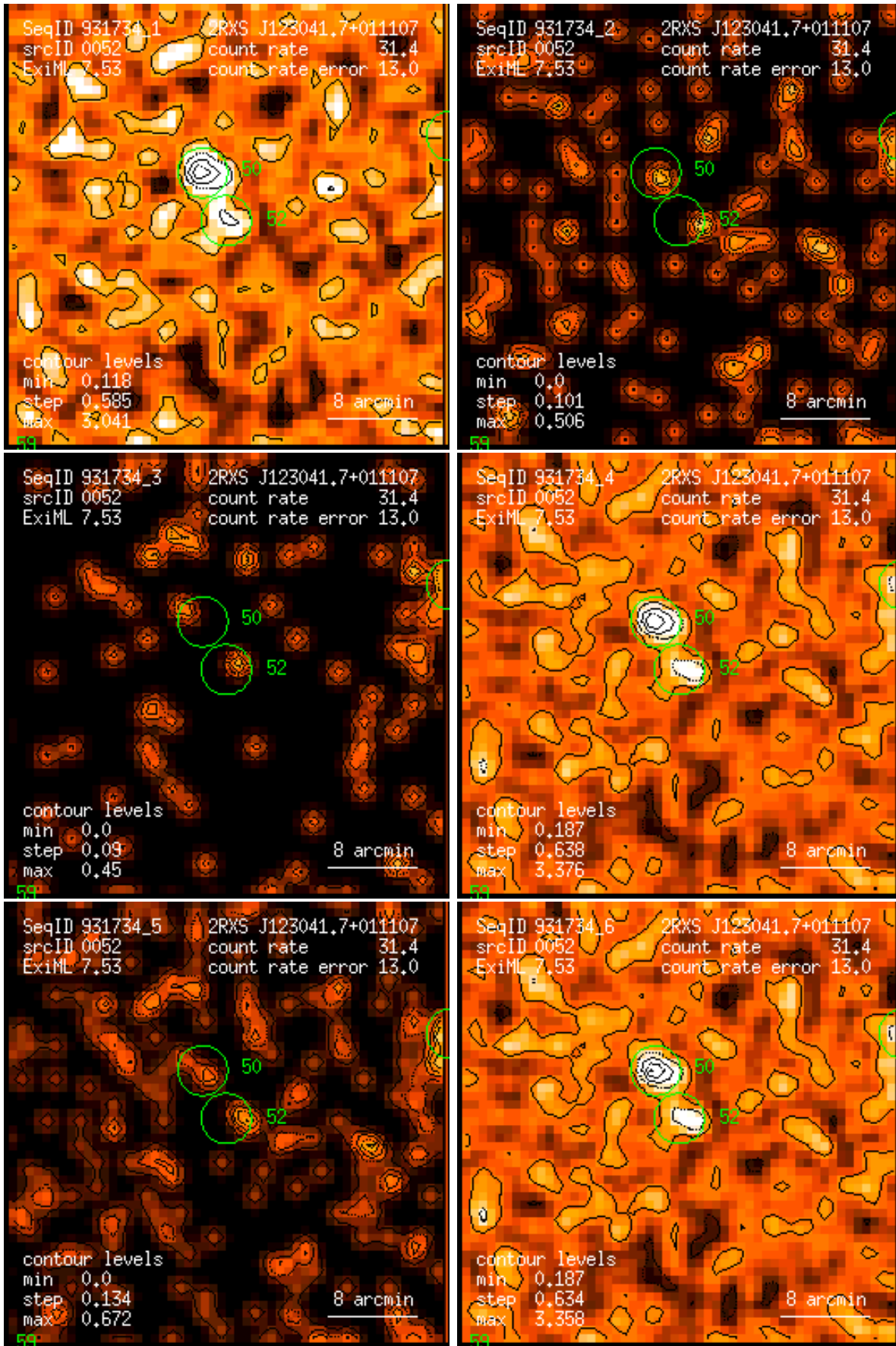
Figure 52: RASS 931734: detection 0052: band rate images, Gaussian filter: (1) PSPC channels 11 – 41, (2) 52 – 90, (3) 91 – 201, (4) 11 – 235, (5) 52 – 201, (6) 11 – 201. Broad band rates in counts/ks. Band rate contour levels in counts/ks/arcmin 2 .
