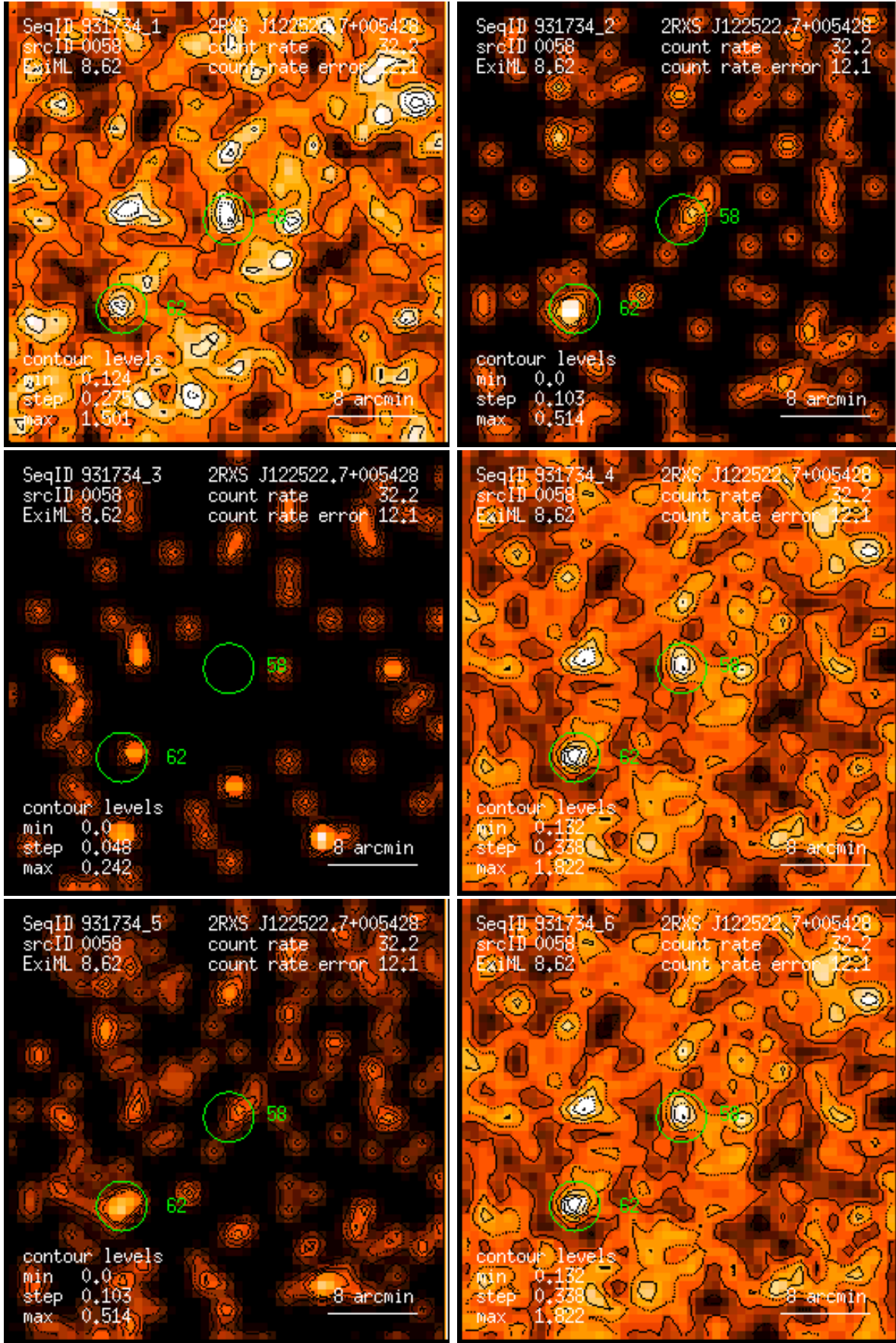
Figure 58: RASS 931734: detection 0058: band rate images, Gaussian filter: (1) PSPC channels 11 – 41, (2) 52 – 90, (3) 91 – 201, (4) 11 – 235, (5) 52 – 201, (6) 11 – 201. Broad band rates in counts/ks. Band rate contour levels in counts/ks/arcmin 2 .
