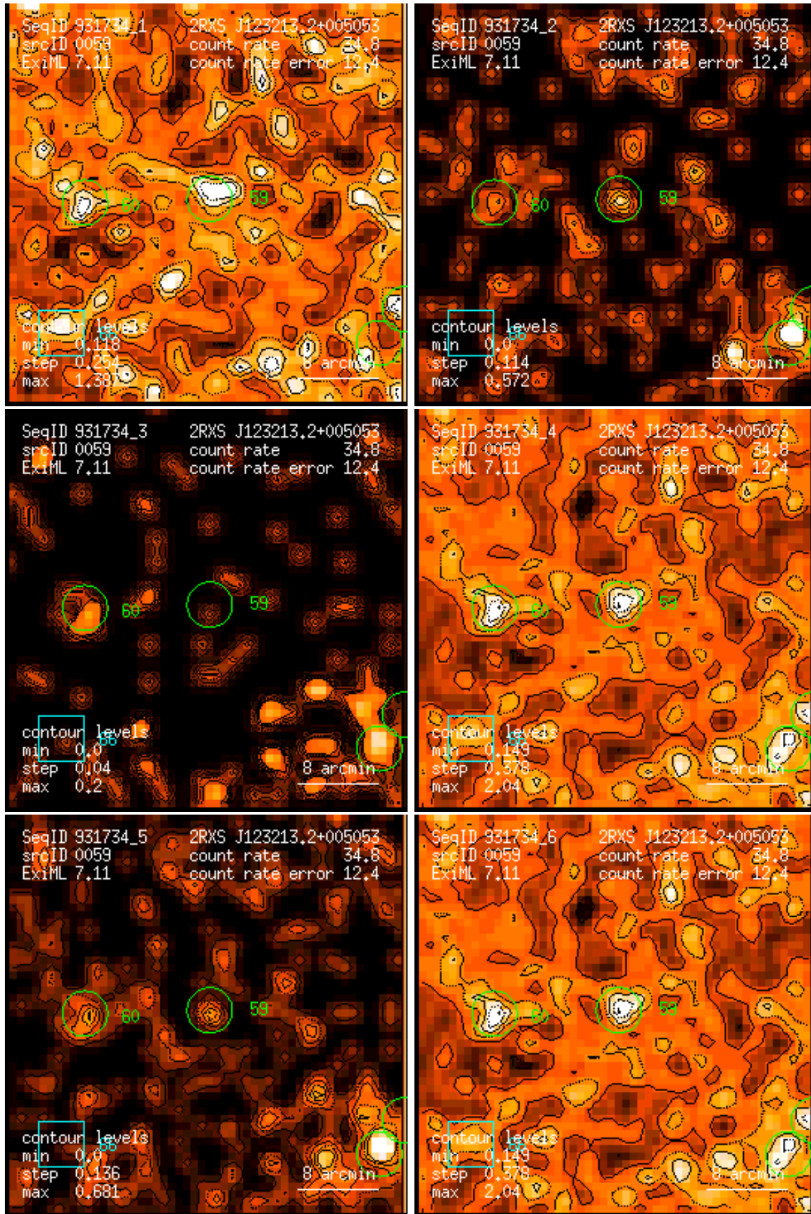
Figure 59: RASS 931734: detection 0059: band rate images, Gaussian filter: (1) PSPC channels 11 – 41, (2) 52 – 90, (3) 91 – 201, (4) 11 – 235, (5) 52 – 201, (6) 11 – 201. Broad band rates in counts/ks. Band rate contour levels in counts/ks/arcmin 2 .
