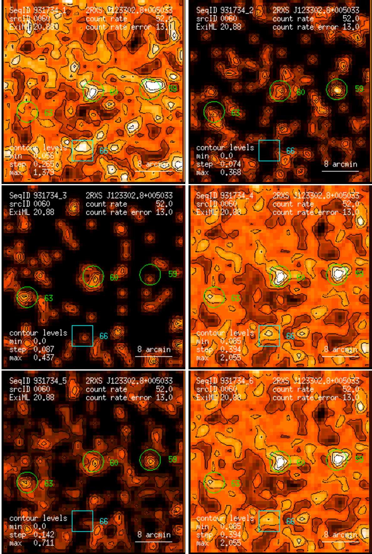
Figure 60: RASS 931734: detection 0060: band rate images, Gaussian filter: (1) PSPC channels 11 – 41, (2) 52 – 90, (3) 91 – 201, (4) 11 – 235, (5) 52 – 201, (6) 11 – 201. Broad band rates in counts/ks. Band rate contour levels in counts/ks/arcmin 2 .
