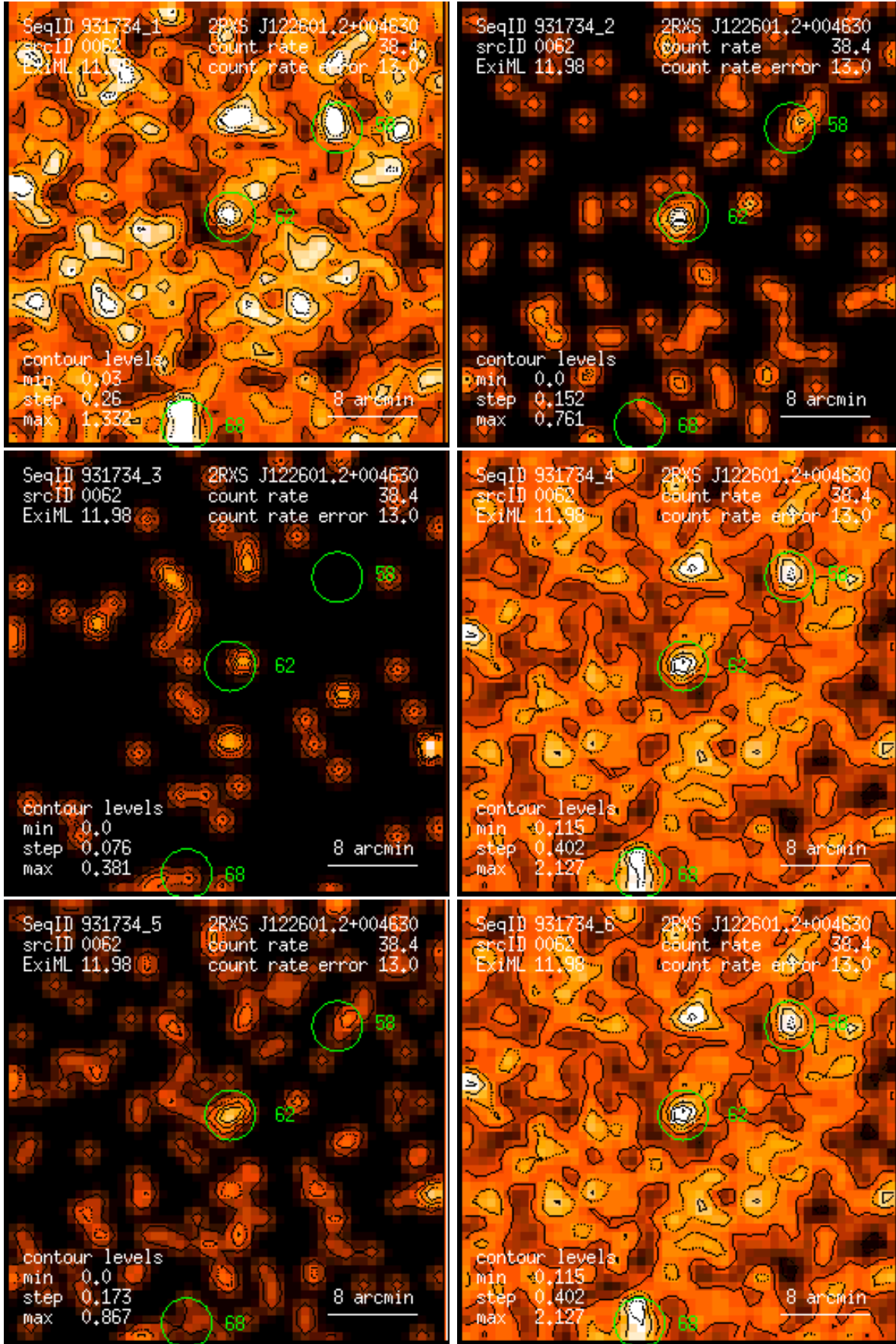
Figure 62: RASS 931734: detection 0062: band rate images, Gaussian filter: (1) PSPC channels 11 – 41, (2) 52 – 90, (3) 91 – 201, (4) 11 – 235, (5) 52 – 201, (6) 11 – 201. Broad band rates in counts/ks. Band rate contour levels in counts/ks/arcmin 2 .
