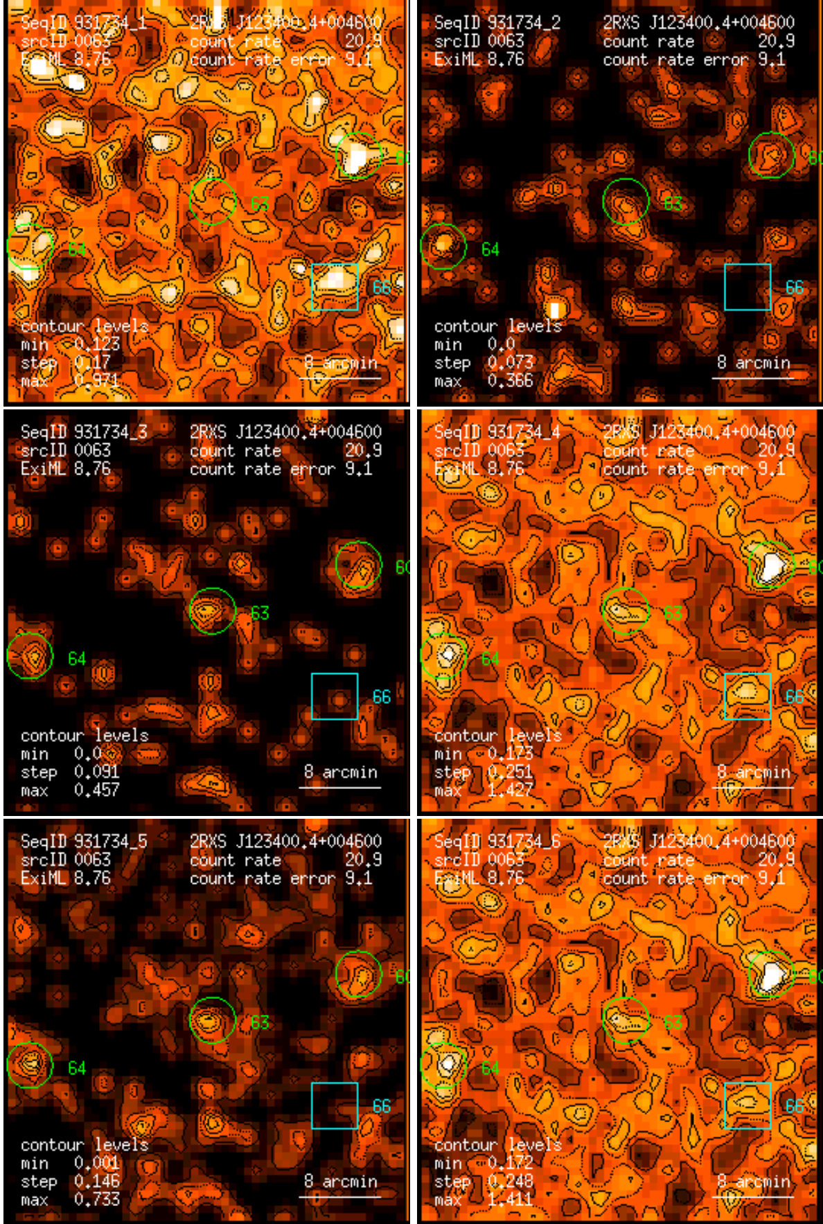
Figure 63: RASS 931734: detection 0063: band rate images, Gaussian filter: (1) PSPC channels 11 – 41, (2) 52 – 90, (3) 91 – 201, (4) 11 – 235, (5) 52 – 201, (6) 11 – 201. Broad band rates in counts/ks. Band rate contour levels in counts/ks/arcmin 2 .
