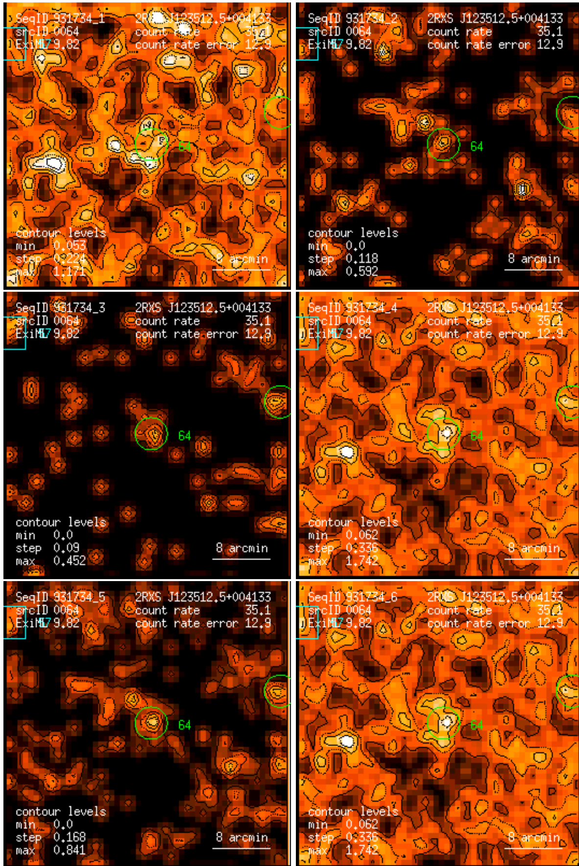
Figure 64: RASS 931734: detection 0064: band rate images, Gaussian filter: (1) PSPC channels 11 – 41, (2) 52 – 90, (3) 91 – 201, (4) 11 – 235, (5) 52 – 201, (6) 11 – 201. Broad band rates in counts/ks. Band rate contour levels in counts/ks/arcmin 2 .
