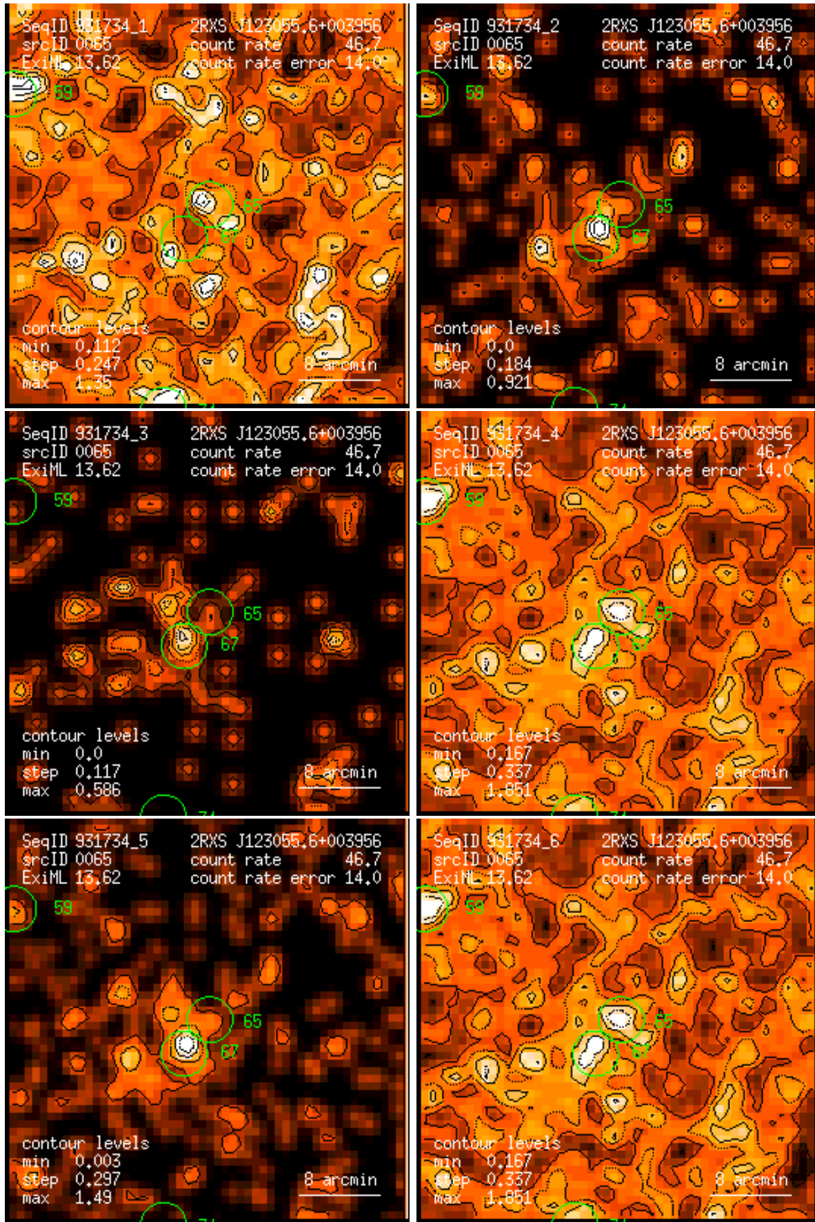
Figure 65: RASS 931734: detection 0065: band rate images, Gaussian filter: (1) PSPC channels 11 – 41, (2) 52 – 90, (3) 91 – 201, (4) 11 – 235, (5) 52 – 201, (6) 11 – 201. Broad band rates in counts/ks. Band rate contour levels in counts/ks/arcmin 2 .
