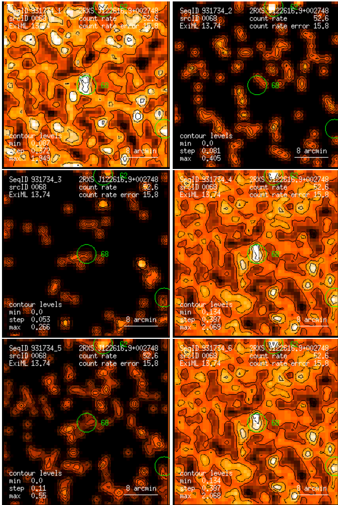
Figure 68: RASS 931734: detection 0068: band rate images, Gaussian filter: (1) PSPC channels 11 – 41, (2) 52 – 90, (3) 91 – 201, (4) 11 – 235, (5) 52 – 201, (6) 11 – 201. Broad band rates in counts/ks. Band rate contour levels in counts/ks/arcmin 2 .
