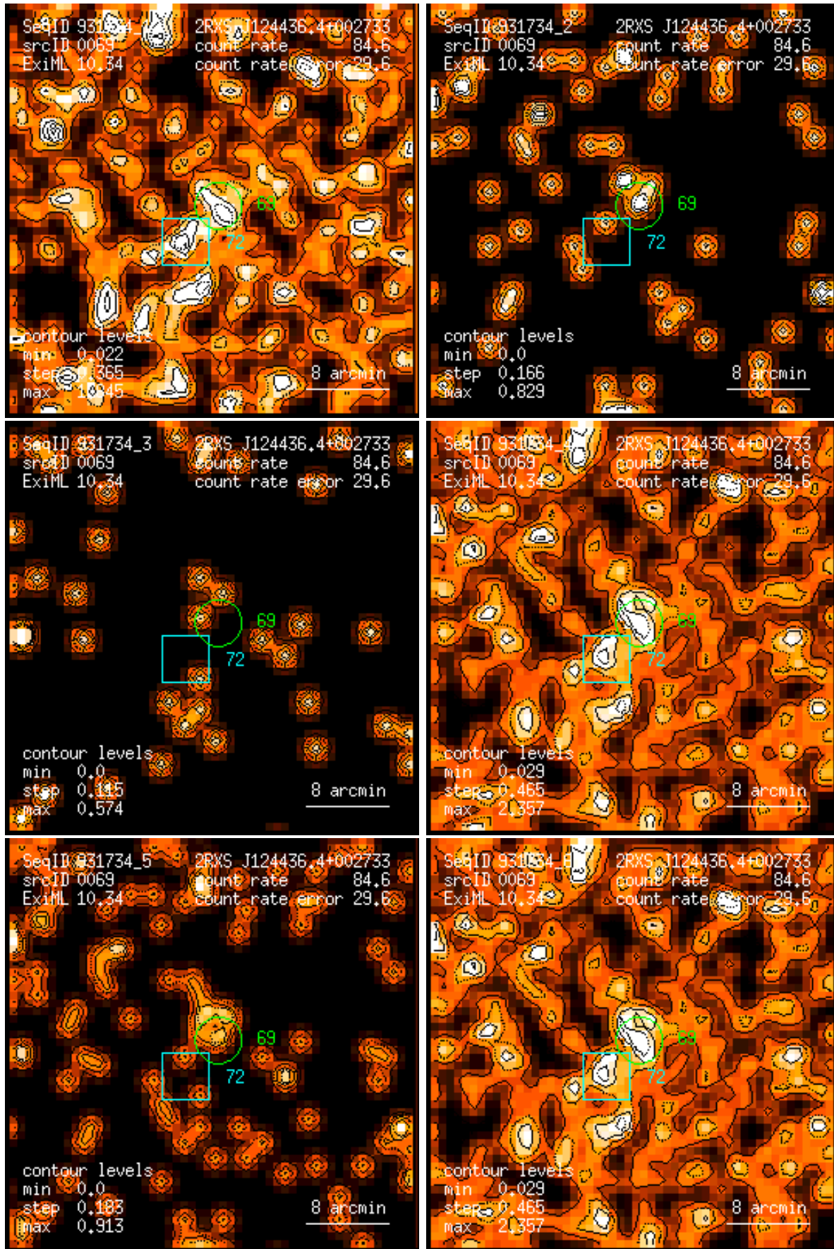
Figure 69: RASS 931734: detection 0069: band rate images, Gaussian filter: (1) PSPC channels 11 – 41, (2) 52 – 90, (3) 91 – 201, (4) 11 – 235, (5) 52 – 201, (6) 11 – 201. Broad band rates in counts/ks. Band rate contour levels in counts/ks/arcmin 2 .
