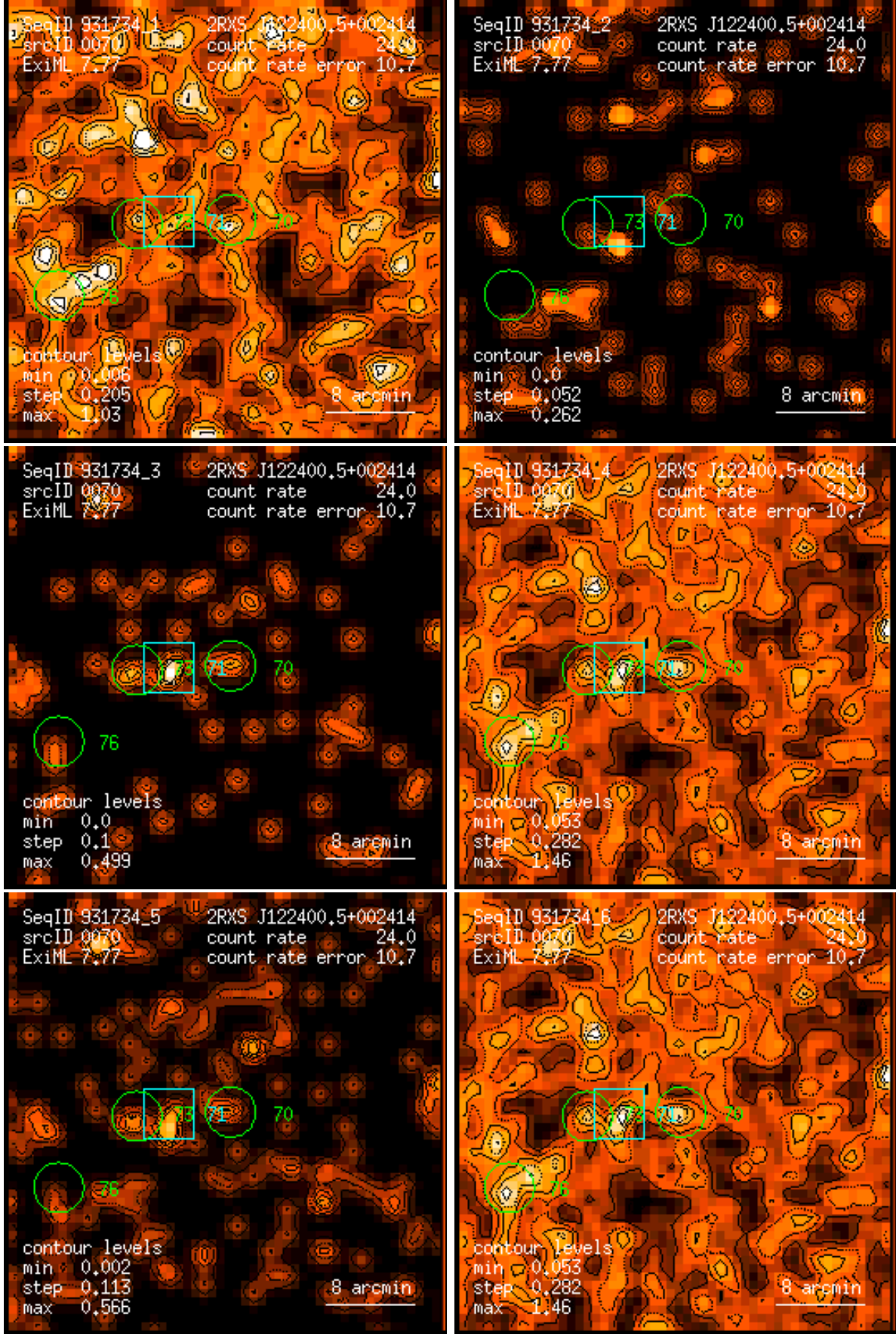
Figure 70: RASS 931734: detection 0070: band rate images, Gaussian filter: (1) PSPC channels 11 – 41, (2) 52 – 90, (3) 91 – 201, (4) 11 – 235, (5) 52 – 201, (6) 11 – 201. Broad band rates in counts/ks. Band rate contour levels in counts/ks/arcmin 2 .
