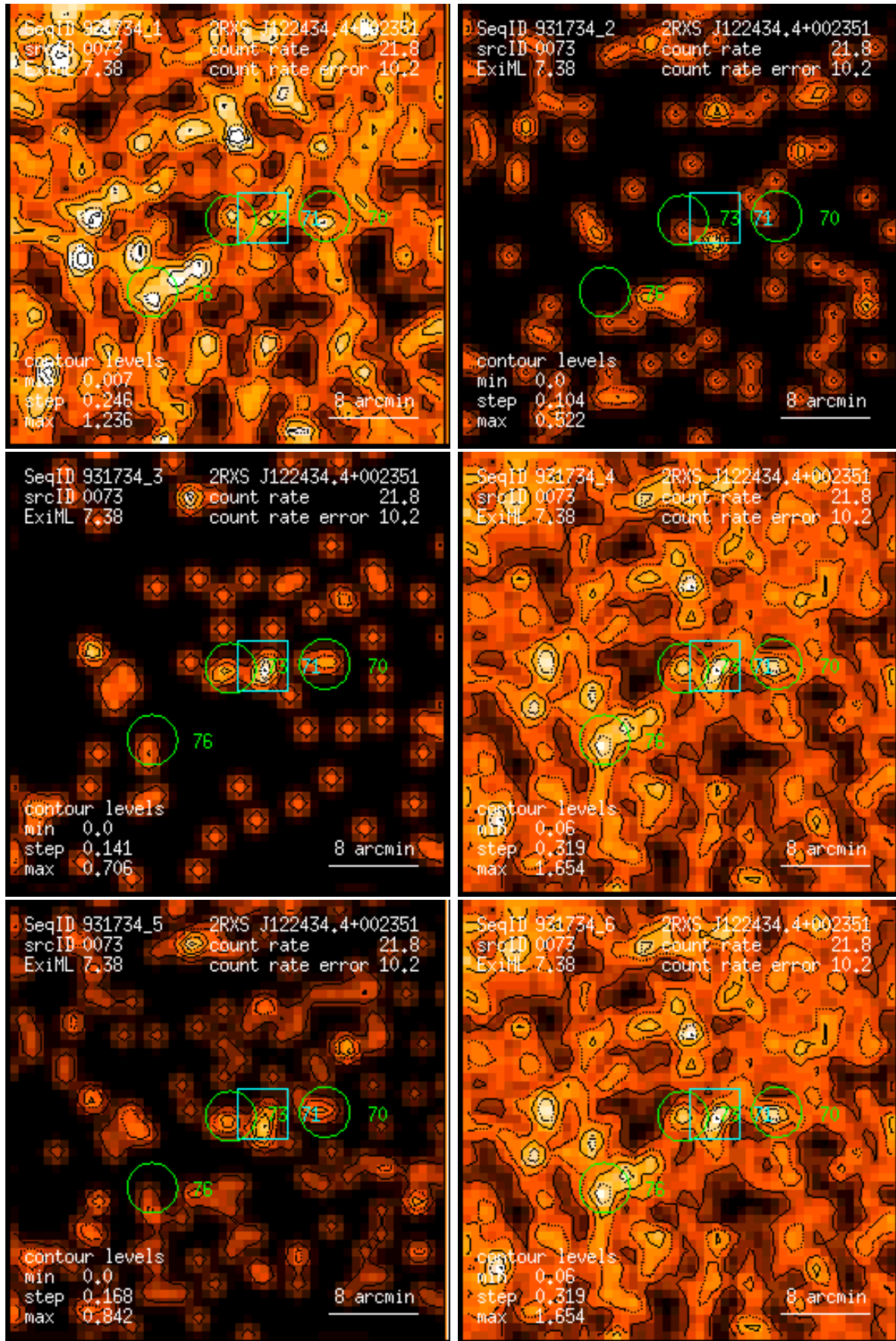
Figure 73: RASS 931734: detection 0073: band rate images, Gaussian filter: (1) PSPC channels 11 – 41, (2) 52 – 90, (3) 91 – 201, (4) 11 – 235, (5) 52 – 201, (6) 11 – 201. Broad band rates in counts/ks. Band rate contour levels in counts/ks/arcmin 2 .
