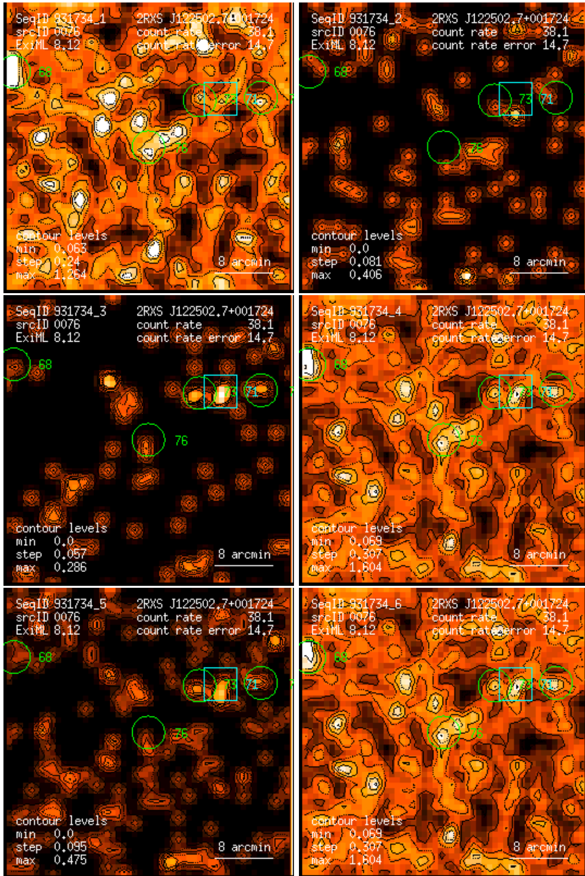
Figure 76: RASS 931734: detection 0076: band rate images, Gaussian filter: (1) PSPC channels 11 – 41, (2) 52 – 90, (3) 91 – 201, (4) 11 – 235, (5) 52 – 201, (6) 11 – 201. Broad band rates in counts/ks. Band rate contour levels in counts/ks/arcmin 2 .
